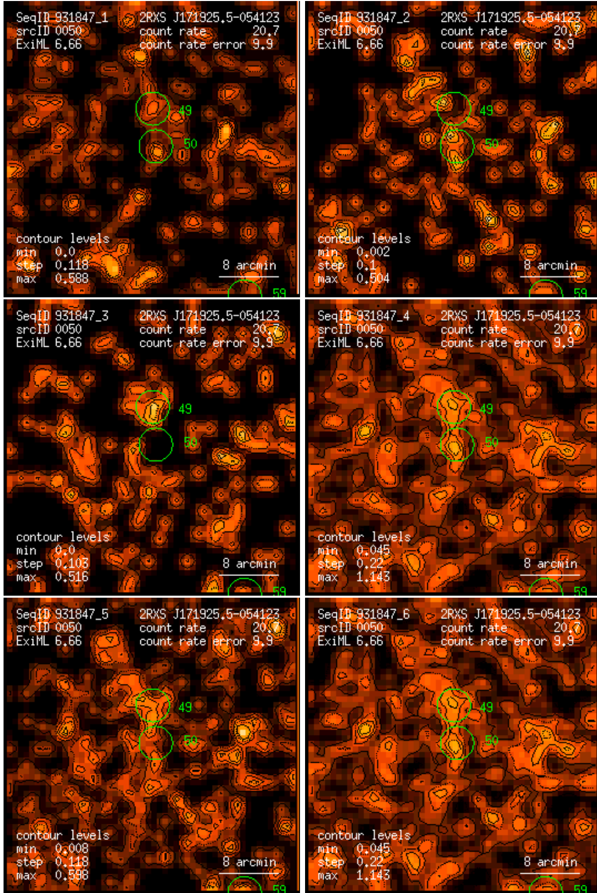
Figure 50: RASS 931847: detection 0050: band rate images, Gaussian filter: (1) PSPC channels 11 – 41, (2) 52 – 90, (3) 91 – 201, (4) 11 – 235, (5) 52 – 201, (6) 11 – 201. Broad band rates in counts/ks. Band rate contour levels in counts/ks/arcmin 2 .
