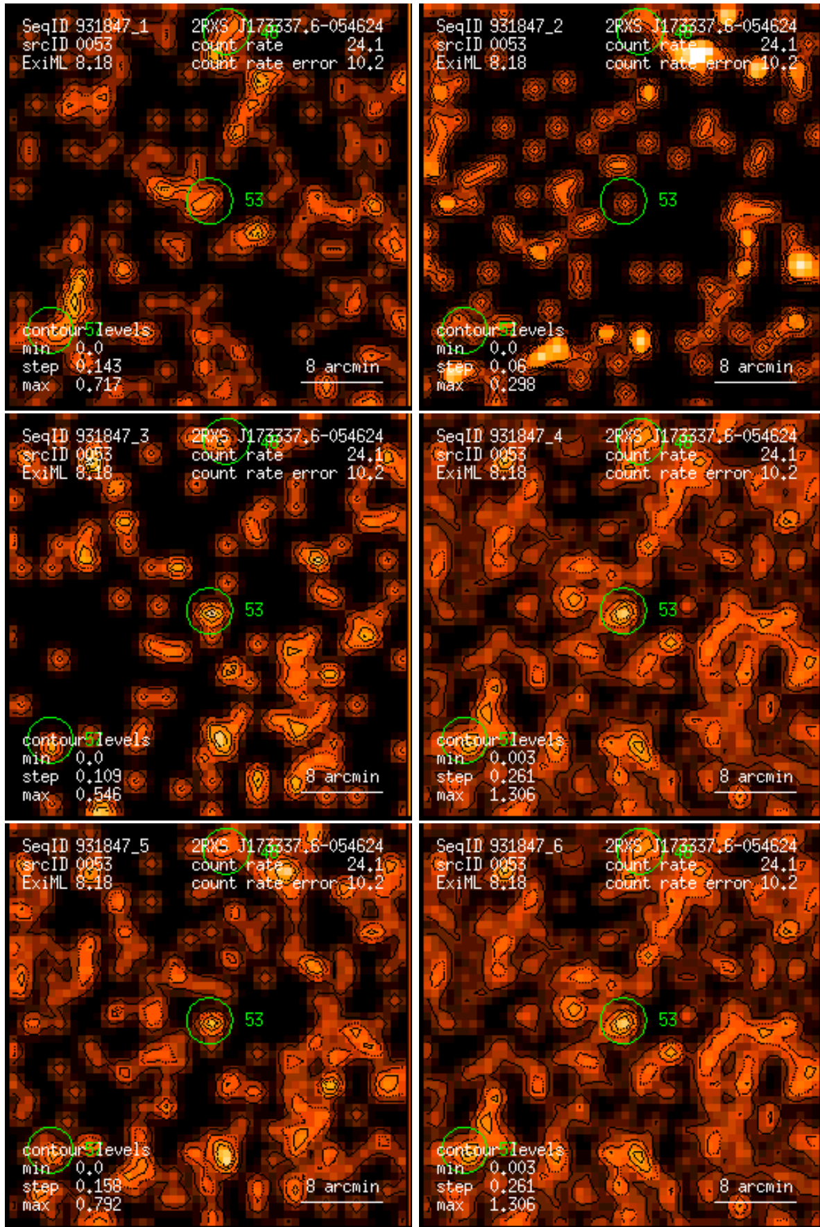
Figure 53: RASS 931847: detection 0053: band rate images, Gaussian filter: (1) PSPC channels 11 – 41, (2) 52 – 90, (3) 91 – 201, (4) 11 – 235, (5) 52 – 201, (6) 11 – 201. Broad band rates in counts/ks. Band rate contour levels in counts/ks/arcmin 2 .
