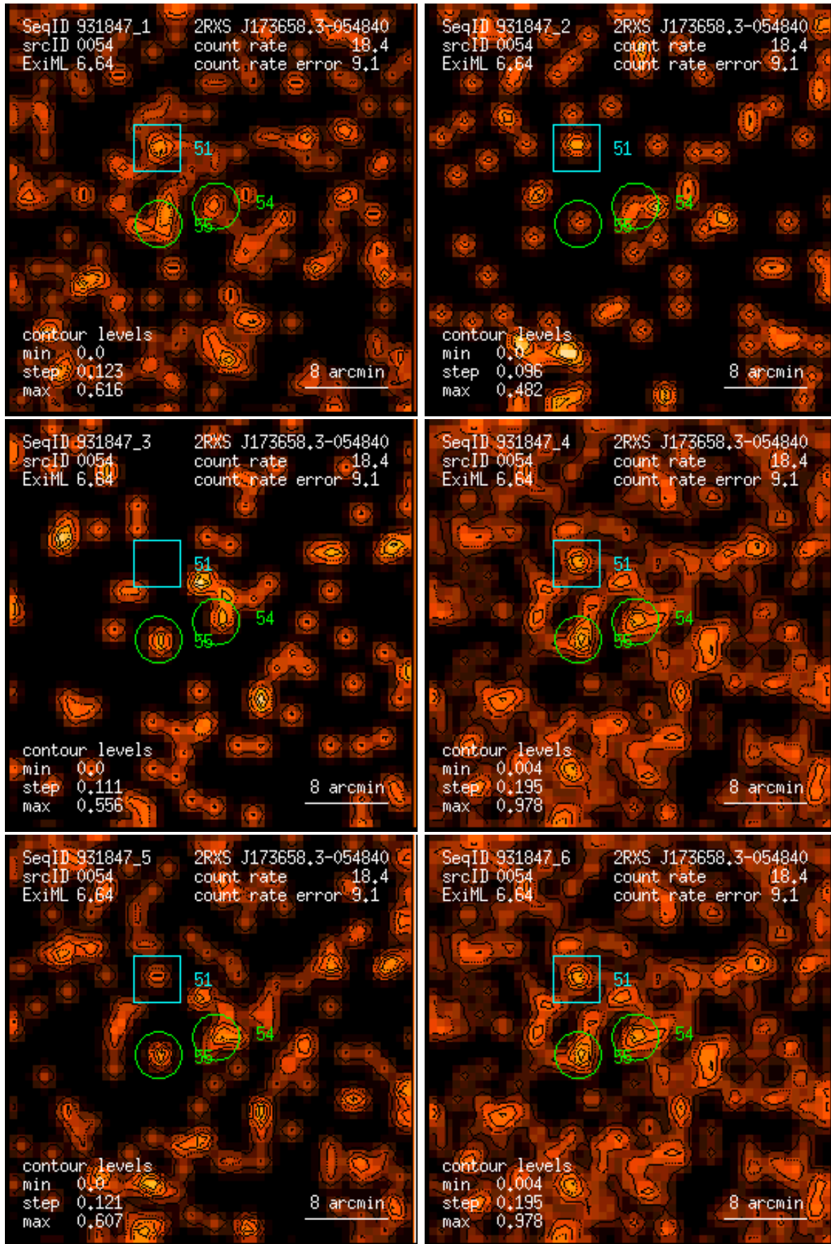
Figure 54: RASS 931847: detection 0054: band rate images, Gaussian filter: (1) PSPC channels 11 – 41, (2) 52 – 90, (3) 91 – 201, (4) 11 – 235, (5) 52 – 201, (6) 11 – 201. Broad band rates in counts/ks. Band rate contour levels in counts/ks/arcmin 2 .
