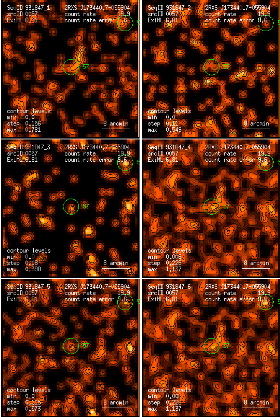
Figure 57: RASS 931847: detection 0057: band rate images, Gaussian filter: (1) PSPC channels 11 – 41, (2) 52 – 90, (3) 91 – 201, (4) 11 – 235, (5) 52 – 201, (6) 11 – 201. Broad band rates in counts/ks. Band rate contour levels in counts/ks/arcmin 2 .
