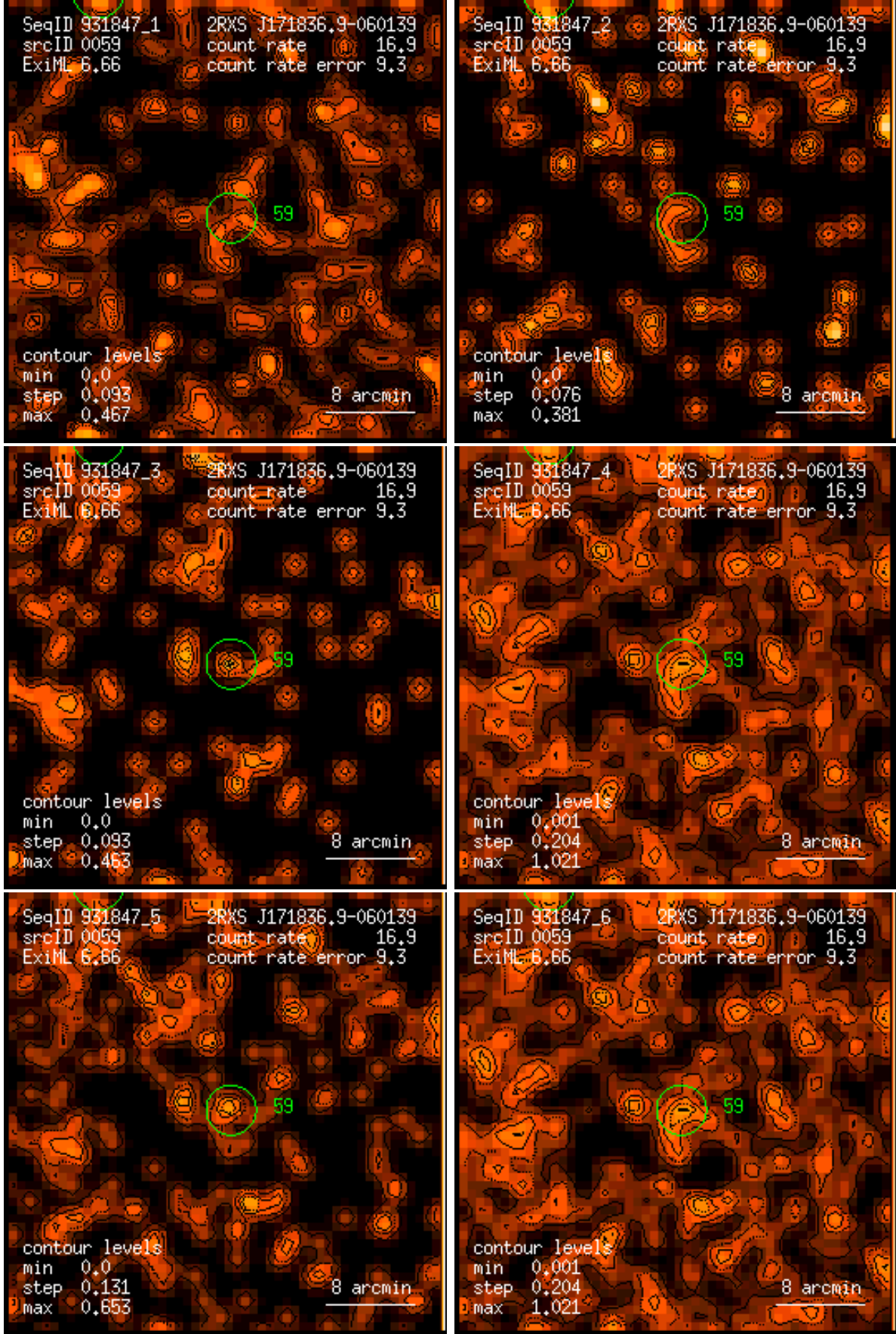
Figure 59: RASS 931847: detection 0059: band rate images, Gaussian filter: (1) PSPC channels 11 – 41, (2) 52 – 90, (3) 91 – 201, (4) 11 – 235, (5) 52 – 201, (6) 11 – 201. Broad band rates in counts/ks. Band rate contour levels in counts/ks/arcmin 2 .
