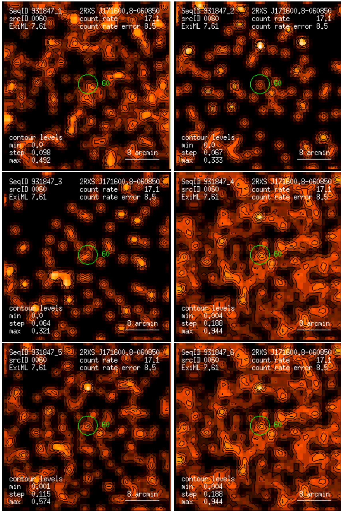
Figure 60: RASS 931847: detection 0060: band rate images, Gaussian filter: (1) PSPC channels 11 – 41, (2) 52 – 90, (3) 91 – 201, (4) 11 – 235, (5) 52 – 201, (6) 11 – 201. Broad band rates in counts/ks. Band rate contour levels in counts/ks/arcmin 2 .
