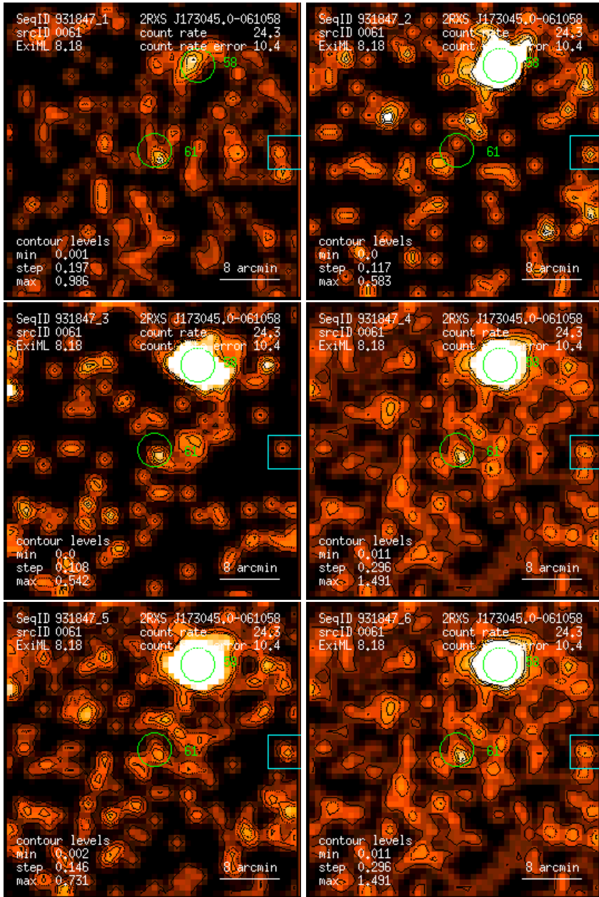
Figure 61: RASS 931847: detection 0061: band rate images, Gaussian filter: (1) PSPC channels 11 – 41, (2) 52 – 90, (3) 91 – 201, (4) 11 – 235, (5) 52 – 201, (6) 11 – 201. Broad band rates in counts/ks. Band rate contour levels in counts/ks/arcmin 2 .
