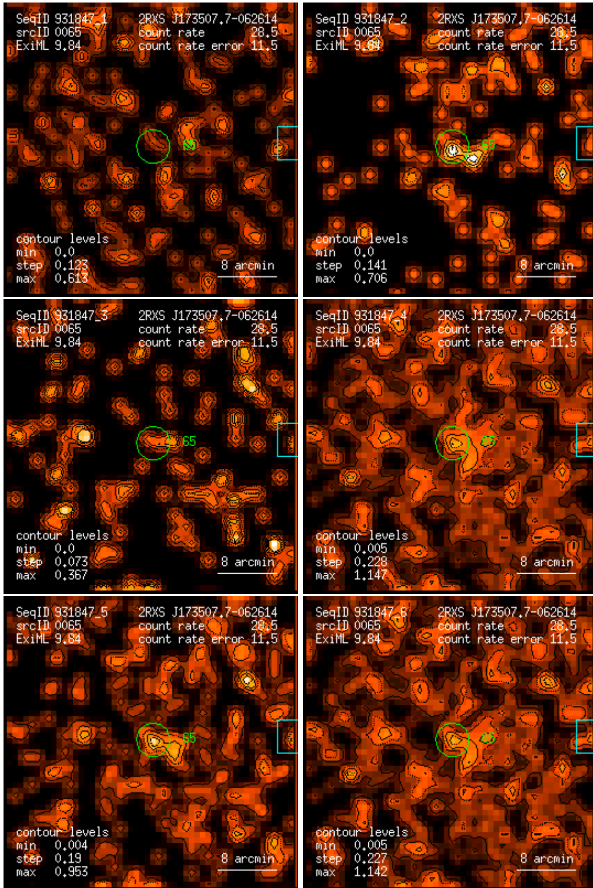
Figure 65: RASS 931847: detection 0065: band rate images, Gaussian filter: (1) PSPC channels 11 – 41, (2) 52 – 90, (3) 91 – 201, (4) 11 – 235, (5) 52 – 201, (6) 11 – 201. Broad band rates in counts/ks. Band rate contour levels in counts/ks/arcmin 2 .
