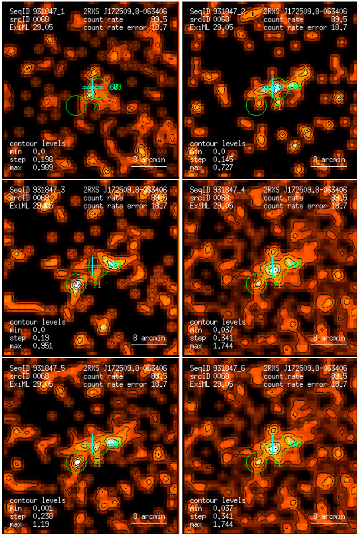
Figure 68: RASS 931847: detection 0068: band rate images, Gaussian filter: (1) PSPC channels 11 – 41, (2) 52 – 90, (3) 91 – 201, (4) 11 – 235, (5) 52 – 201, (6) 11 – 201. Broad band rates in counts/ks. Band rate contour levels in counts/ks/arcmin 2 .
