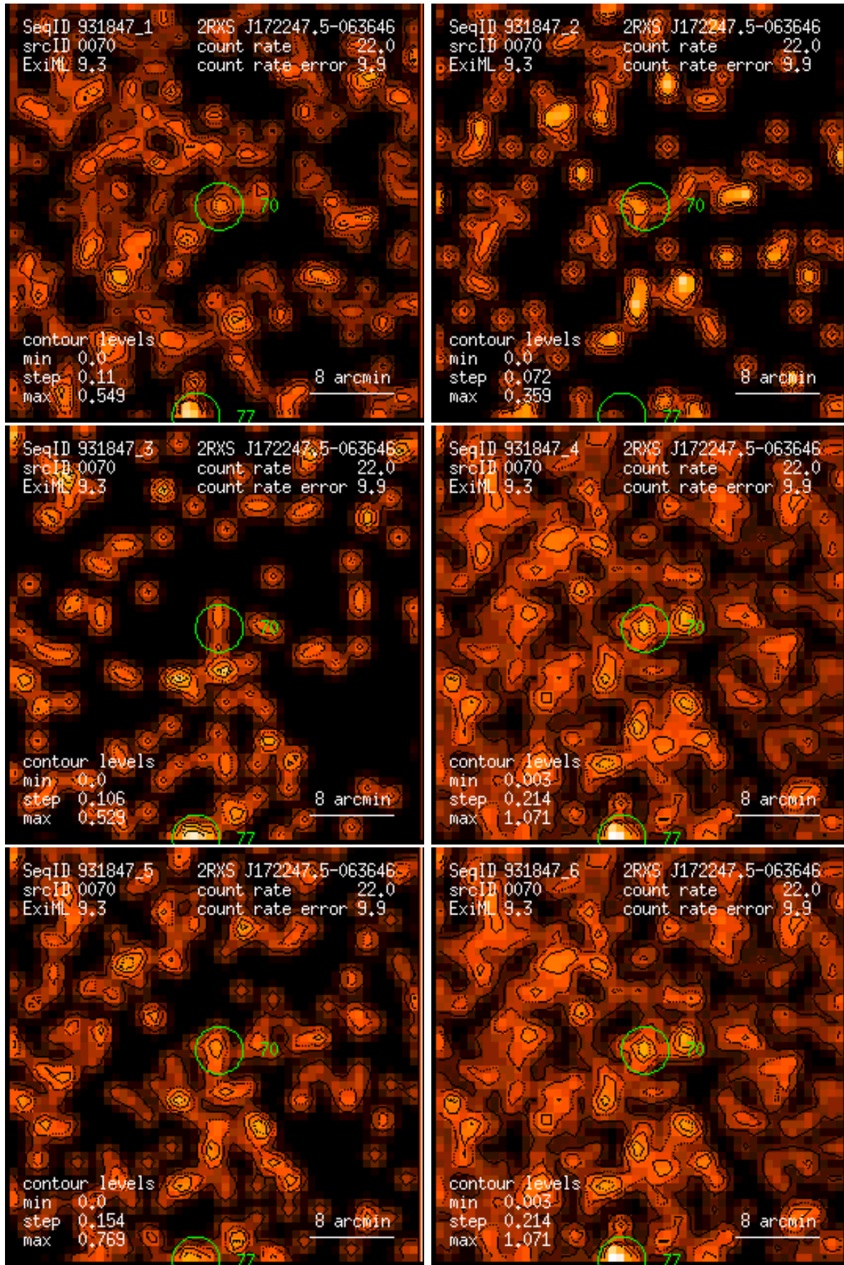
Figure 70: RASS 931847: detection 0070: band rate images, Gaussian filter: (1) PSPC channels 11 – 41, (2) 52 – 90, (3) 91 – 201, (4) 11 – 235, (5) 52 – 201, (6) 11 – 201. Broad band rates in counts/ks. Band rate contour levels in counts/ks/arcmin 2 .
