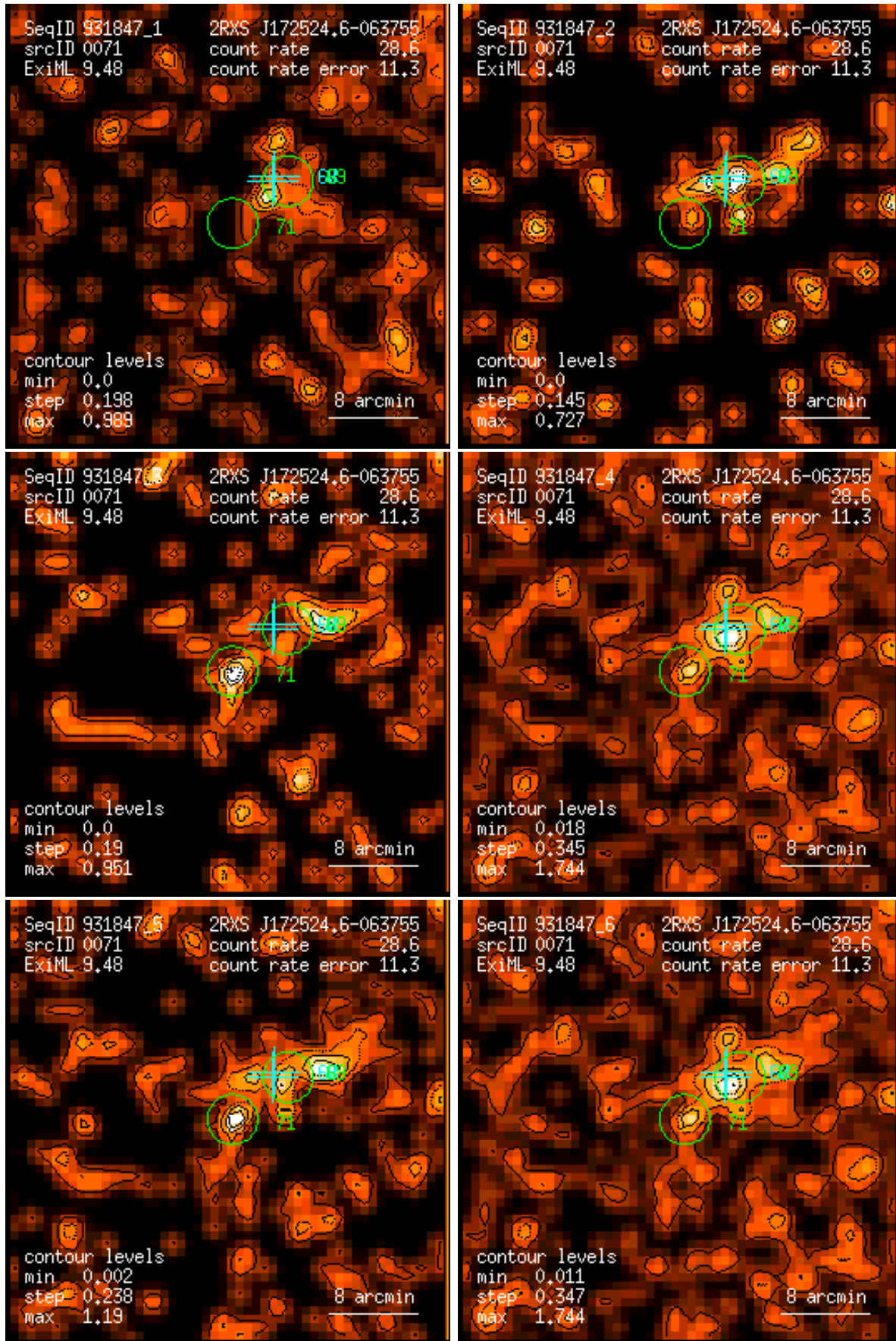
Figure 71: RASS 931847: detection 0071: band rate images, Gaussian filter: (1) PSPC channels 11 – 41, (2) 52 – 90, (3) 91 – 201, (4) 11 – 235, (5) 52 – 201, (6) 11 – 201. Broad band rates in counts/ks. Band rate contour levels in counts/ks/arcmin 2 .
