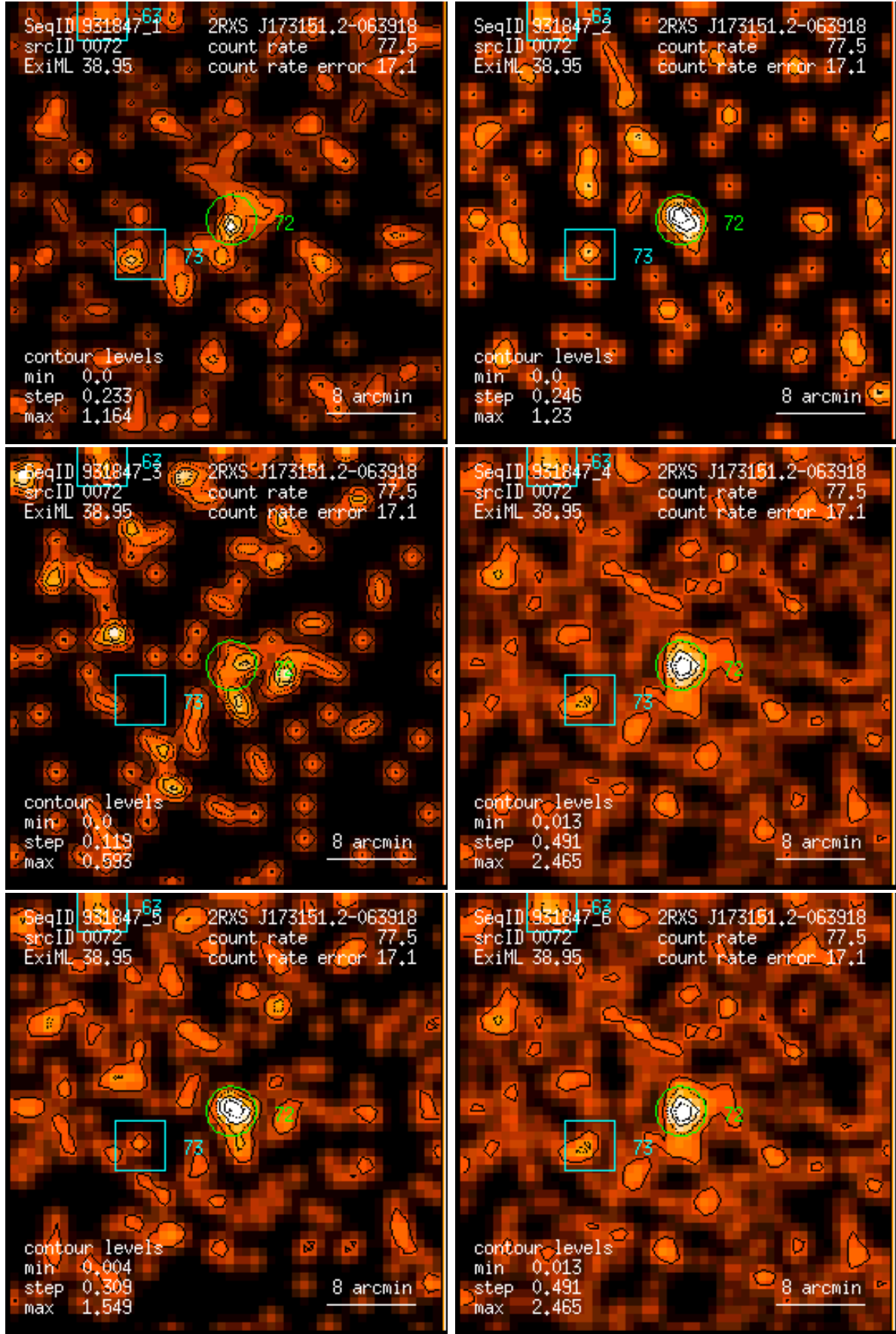
Figure 72: RASS 931847: detection 0072: band rate images, Gaussian filter: (1) PSPC channels 11 – 41, (2) 52 – 90, (3) 91 – 201, (4) 11 – 235, (5) 52 – 201, (6) 11 – 201. Broad band rates in counts/ks. Band rate contour levels in counts/ks/arcmin 2 .
