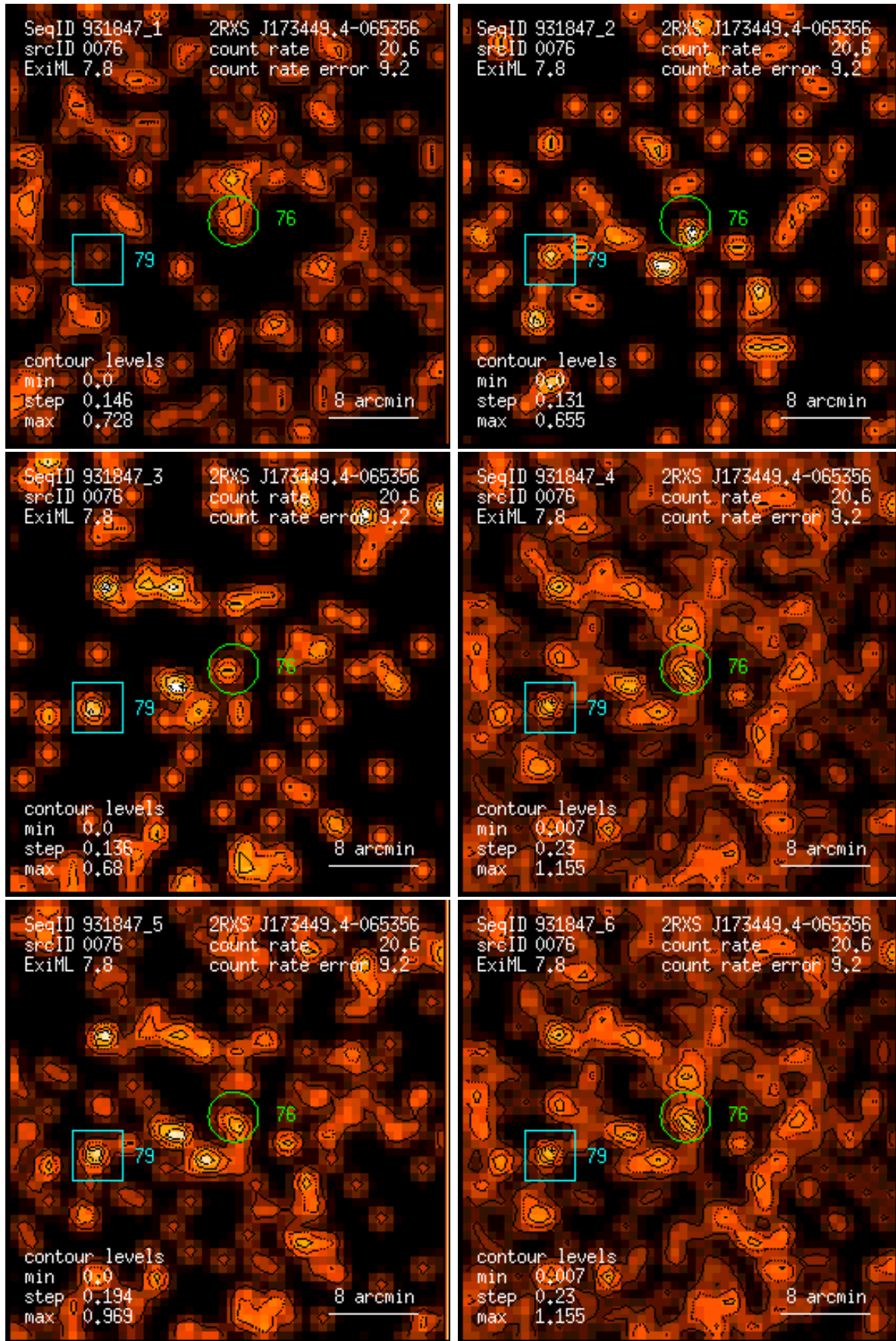
Figure 76: RASS 931847: detection 0076: band rate images, Gaussian filter: (1) PSPC channels 11 – 41, (2) 52 – 90, (3) 91 – 201, (4) 11 – 235, (5) 52 – 201, (6) 11 – 201. Broad band rates in counts/ks. Band rate contour levels in counts/ks/arcmin 2 .
