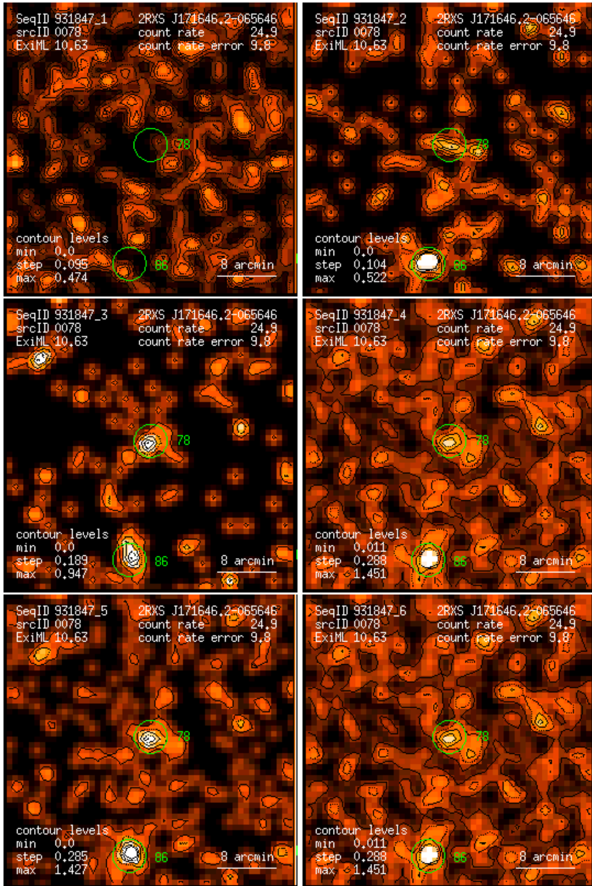
Figure 78: RASS 931847: detection 0078: band rate images, Gaussian filter: (1) PSPC channels 11 – 41, (2) 52 – 90, (3) 91 – 201, (4) 11 – 235, (5) 52 – 201, (6) 11 – 201. Broad band rates in counts/ks. Band rate contour levels in counts/ks/arcmin 2 .
