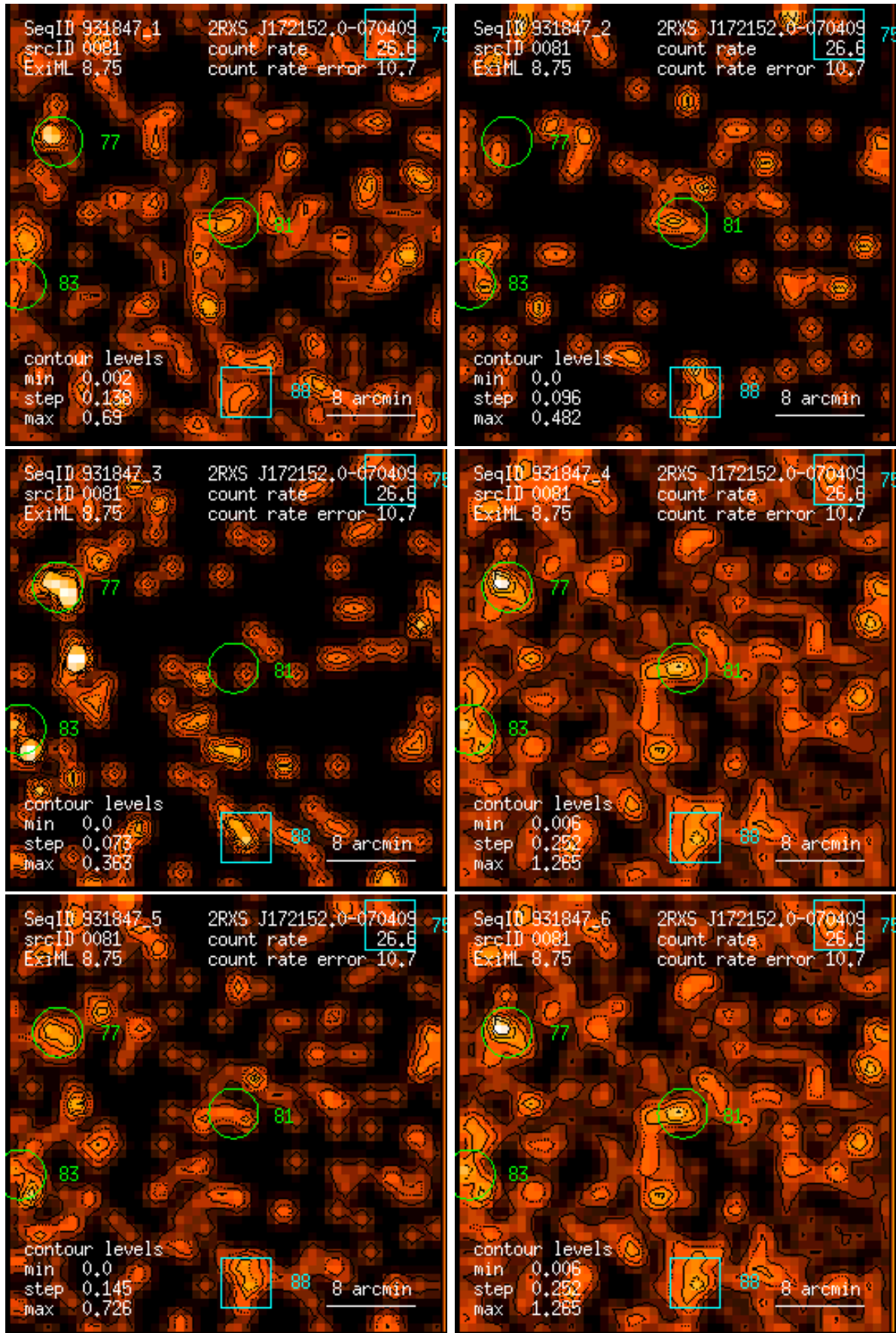
Figure 81: RASS 931847: detection 0081: band rate images, Gaussian filter: (1) PSPC channels 11 – 41, (2) 52 – 90, (3) 91 – 201, (4) 11 – 235, (5) 52 – 201, (6) 11 – 201. Broad band rates in counts/ks. Band rate contour levels in counts/ks/arcmin 2 .
