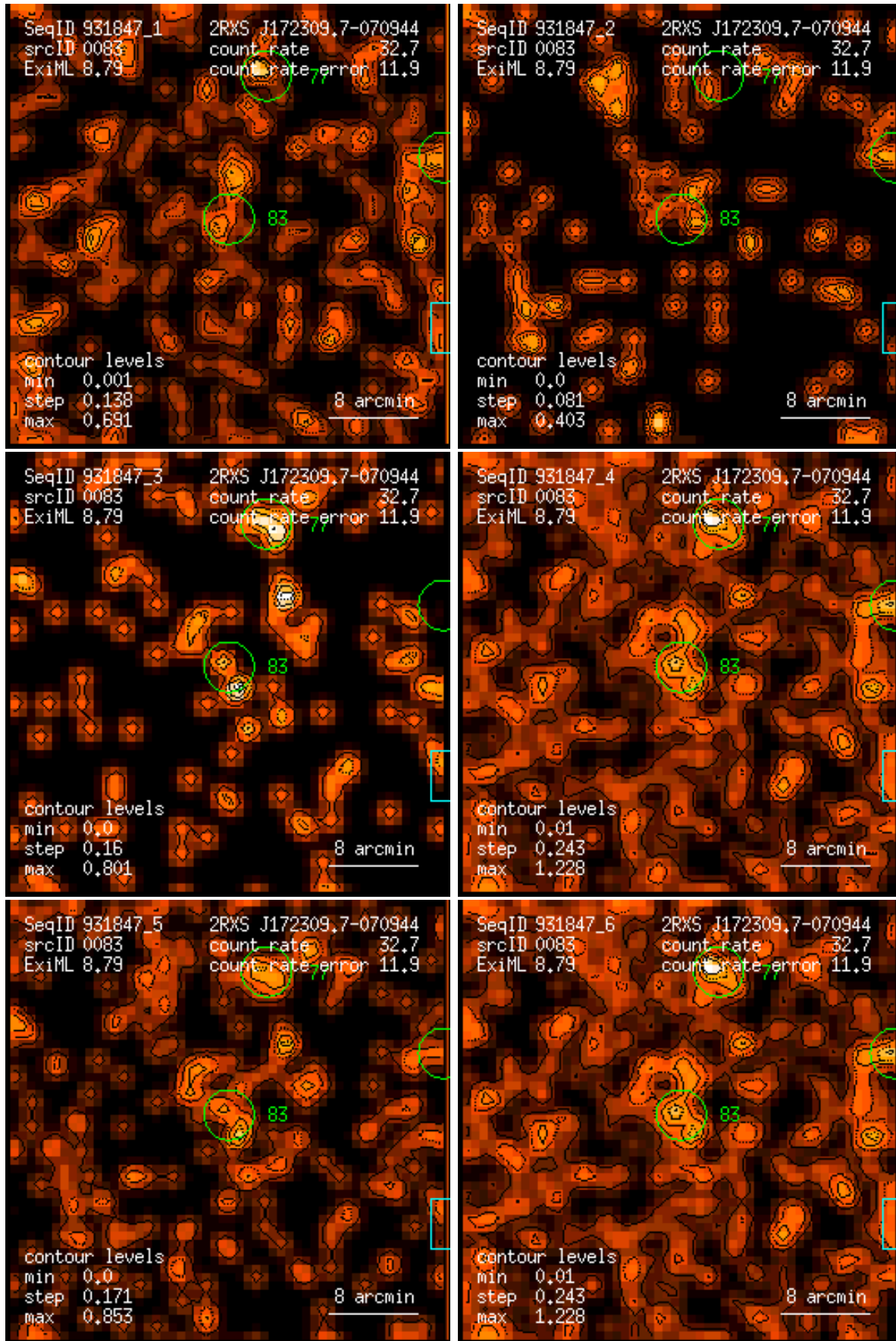
Figure 83: RASS 931847: detection 0083: band rate images, Gaussian filter: (1) PSPC channels 11 – 41, (2) 52 – 90, (3) 91 – 201, (4) 11 – 235, (5) 52 – 201, (6) 11 – 201. Broad band rates in counts/ks. Band rate contour levels in counts/ks/arcmin 2 .
