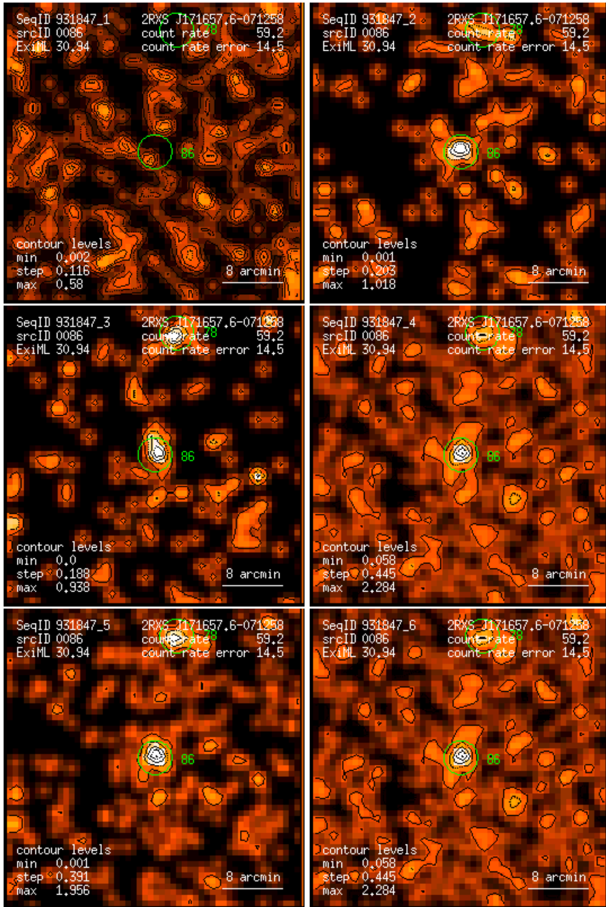
Figure 86: RASS 931847: detection 0086: band rate images, Gaussian filter: (1) PSPC channels 11 – 41, (2) 52 – 90, (3) 91 – 201, (4) 11 – 235, (5) 52 – 201, (6) 11 – 201. Broad band rates in counts/ks. Band rate contour levels in counts/ks/arcmin 2 .
