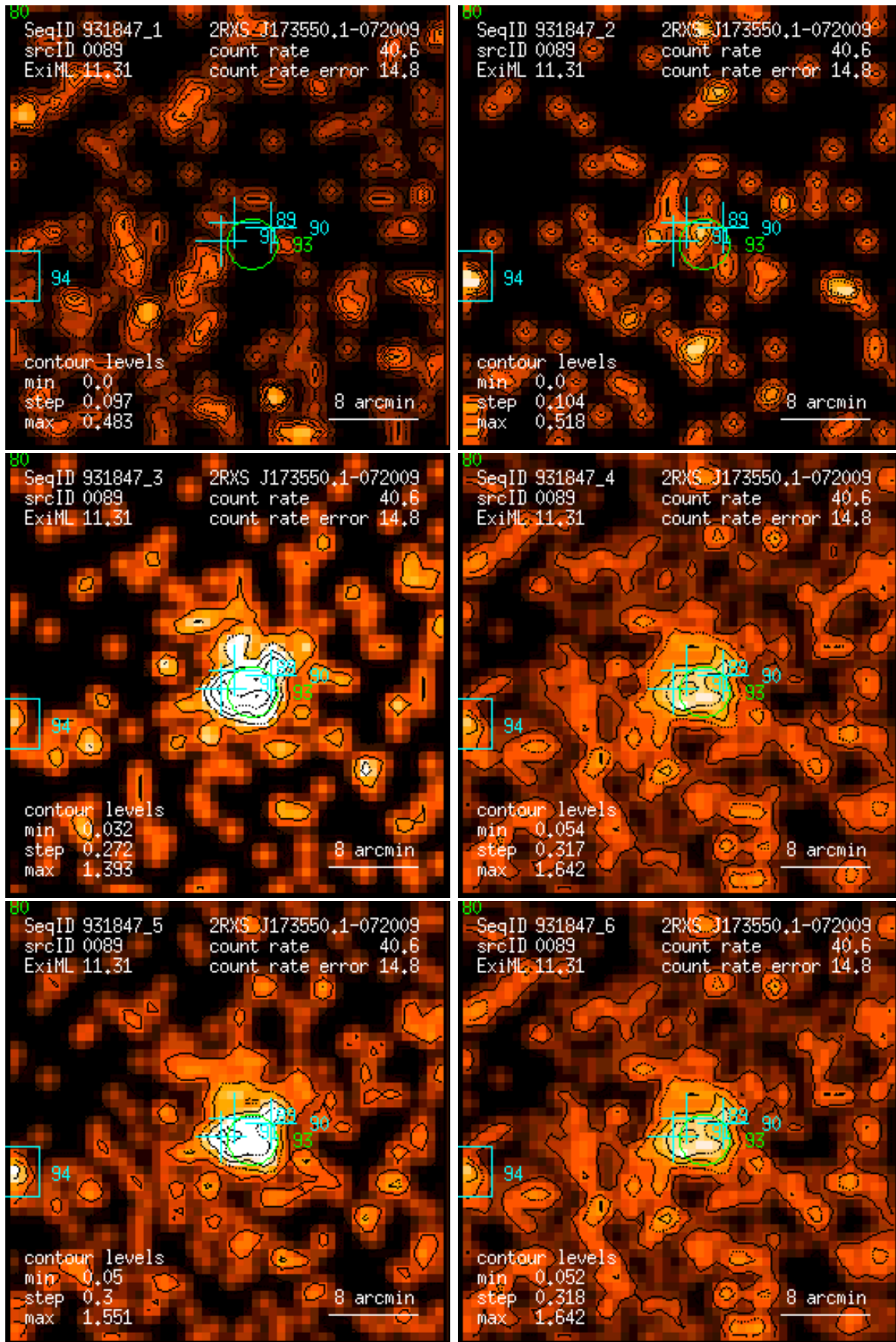
Figure 89: RASS 931847: detection 0089: band rate images, Gaussian filter: (1) PSPC channels 11 – 41, (2) 52 – 90, (3) 91 – 201, (4) 11 – 235, (5) 52 – 201, (6) 11 – 201. Broad band rates in counts/ks. Band rate contour levels in counts/ks/arcmin 2 .
