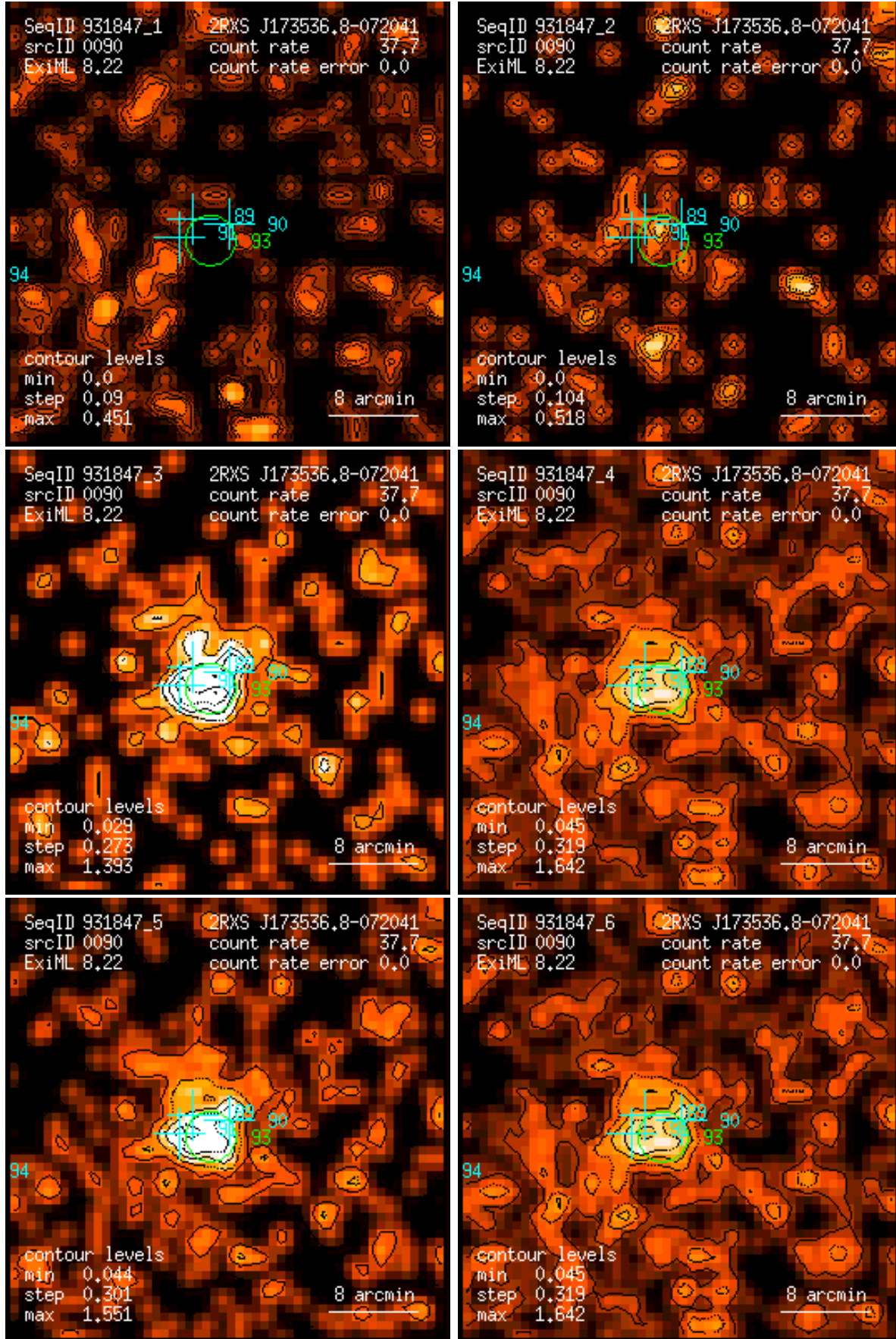
Figure 90: RASS 931847: detection 0090: band rate images, Gaussian filter: (1) PSPC channels 11 – 41, (2) 52 – 90, (3) 91 – 201, (4) 11 – 235, (5) 52 – 201, (6) 11 – 201. Broad band rates in counts/ks. Band rate contour levels in counts/ks/arcmin 2 .
