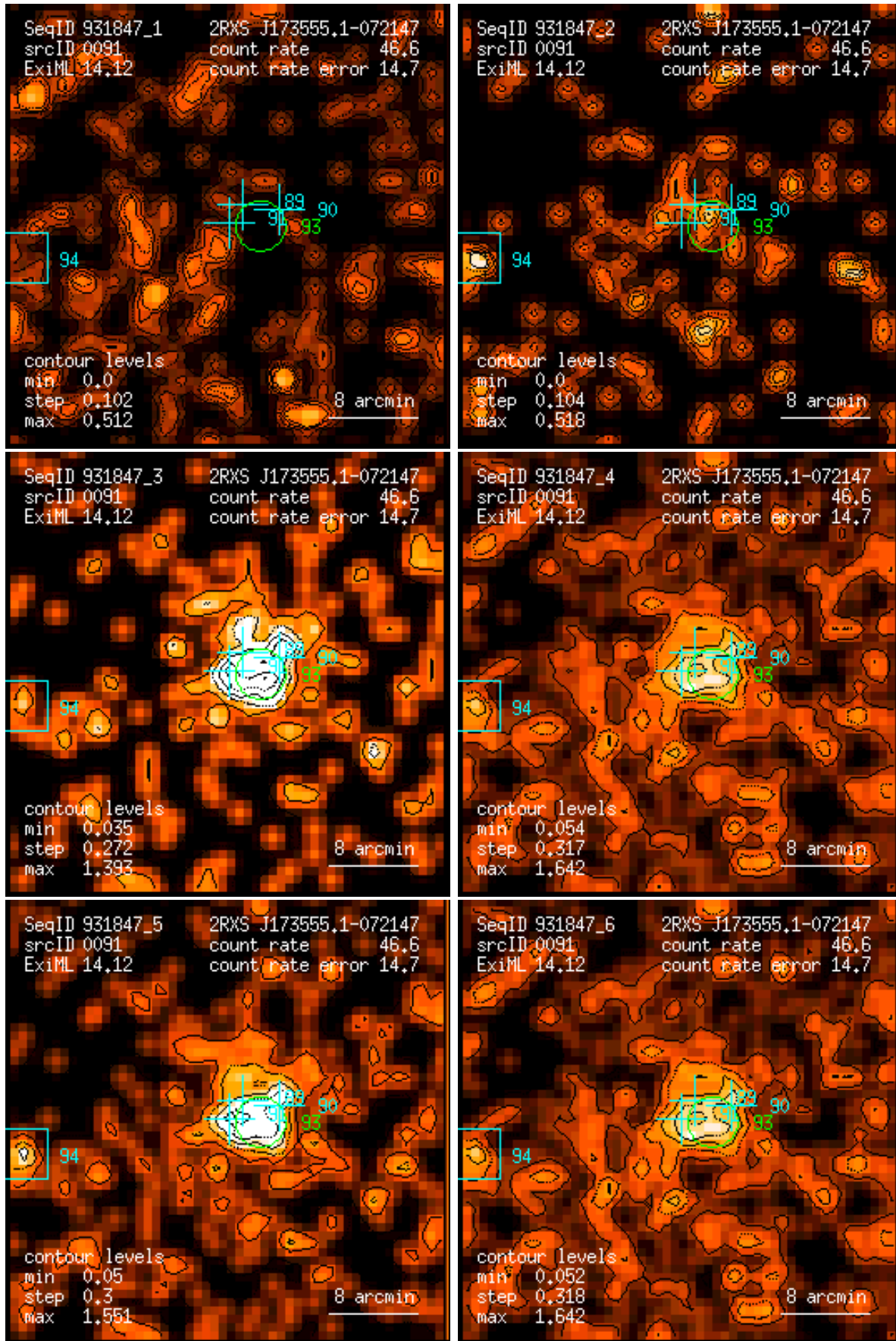
Figure 91: RASS 931847: detection 0091: band rate images, Gaussian filter: (1) PSPC channels 11 – 41, (2) 52 – 90, (3) 91 – 201, (4) 11 – 235, (5) 52 – 201, (6) 11 – 201. Broad band rates in counts/ks. Band rate contour levels in counts/ks/arcmin 2 .
