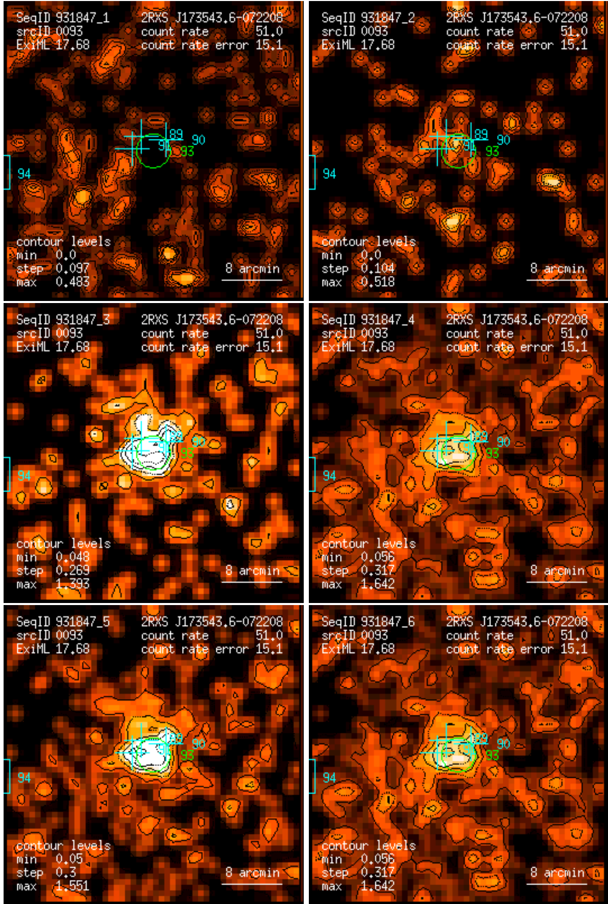
Figure 93: RASS 931847: detection 0093: band rate images, Gaussian filter: (1) PSPC channels 11 – 41, (2) 52 – 90, (3) 91 – 201, (4) 11 – 235, (5) 52 – 201, (6) 11 – 201. Broad band rates in counts/ks. Band rate contour levels in counts/ks/arcmin 2 .
