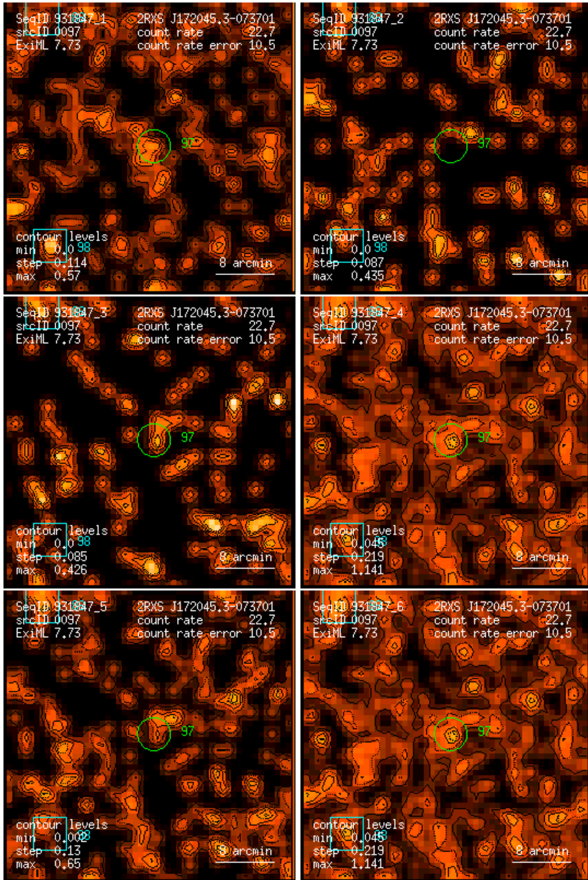
Figure 97: RASS 931847: detection 0097: band rate images, Gaussian filter: (1) PSPC channels 11 – 41, (2) 52 – 90, (3) 91 – 201, (4) 11 – 235, (5) 52 – 201, (6) 11 – 201. Broad band rates in counts/ks. Band rate contour levels in counts/ks/arcmin 2 .
