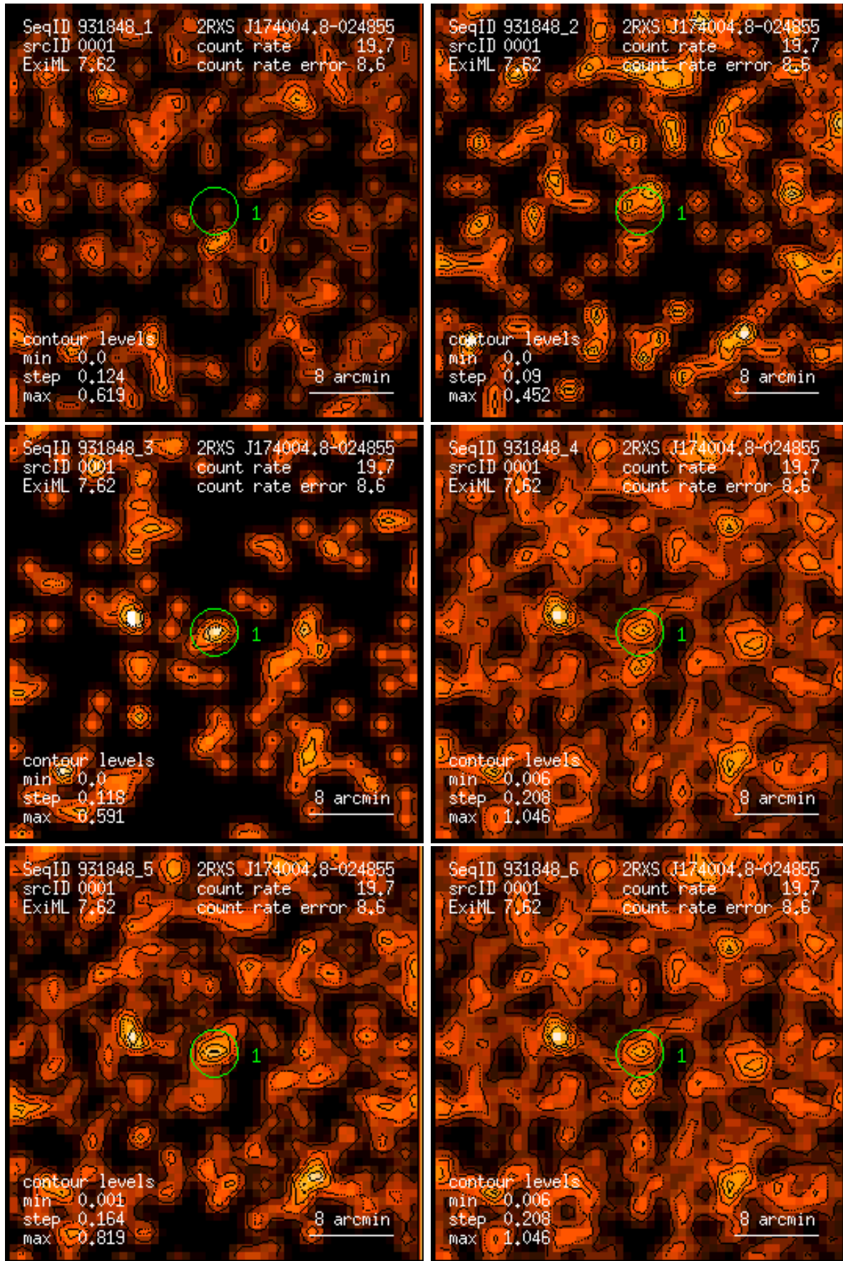
Figure 1: RASS 931848: detection 0001: band rate images, Gaussian filter: (1) PSPC channels 11 – 41, (2) 52 – 90, (3) 91 – 201, (4) 11 – 235, (5) 52 – 201, (6) 11 – 201. Broad band rates in counts/ks. Band rate contour levels in counts/ks/arcmin 2 .
