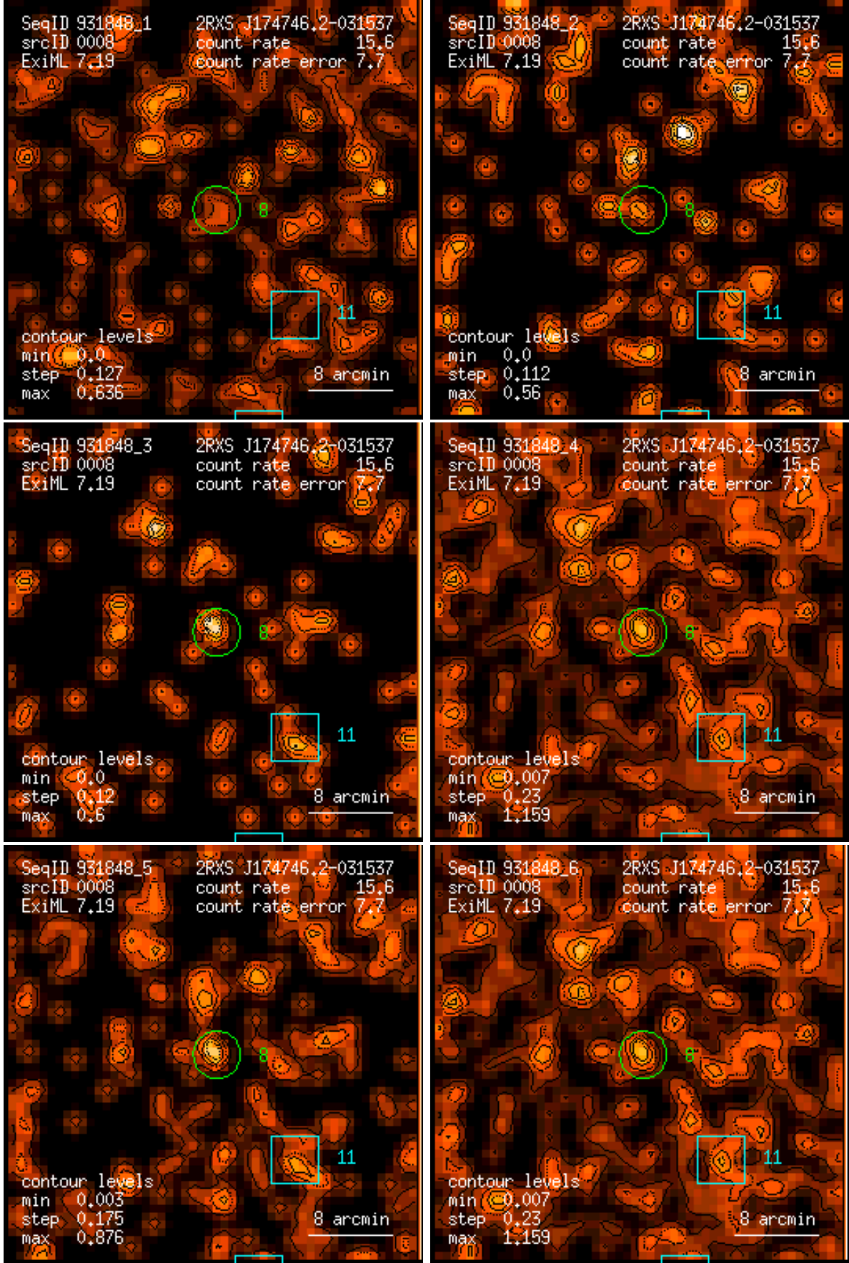
Figure 8: RASS 931848: detection 0008: band rate images, Gaussian filter: (1) PSPC channels 11 – 41, (2) 52 – 90, (3) 91 – 201, (4) 11 – 235, (5) 52 – 201, (6) 11 – 201. Broad band rates in counts/ks. Band rate contour levels in counts/ks/arcmin 2 .
