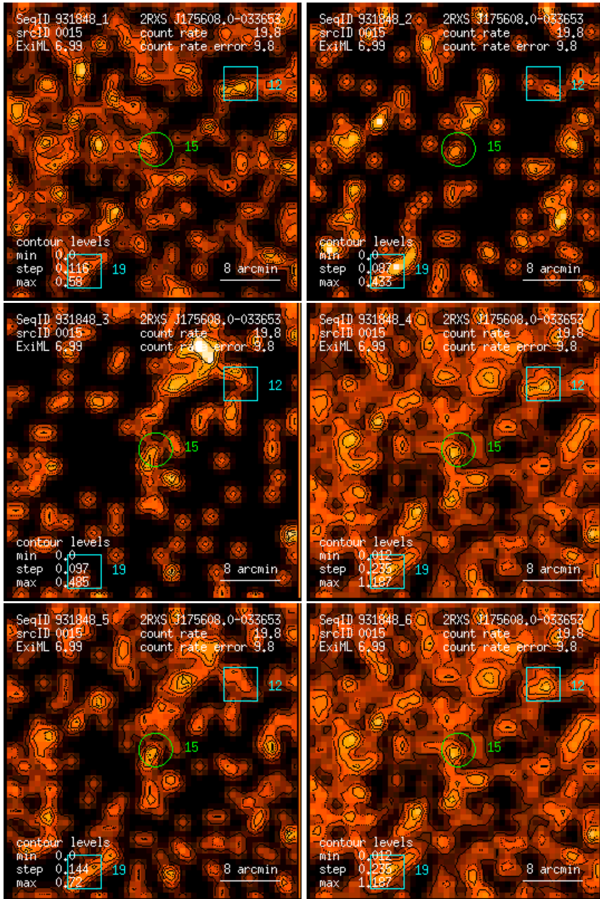
Figure 15: RASS 931848: detection 0015: band rate images, Gaussian filter: (1) PSPC channels 11 – 41, (2) 52 – 90, (3) 91 – 201, (4) 11 – 235, (5) 52 – 201, (6) 11 – 201. Broad band rates in counts/ks. Band rate contour levels in counts/ks/arcmin 2 .
