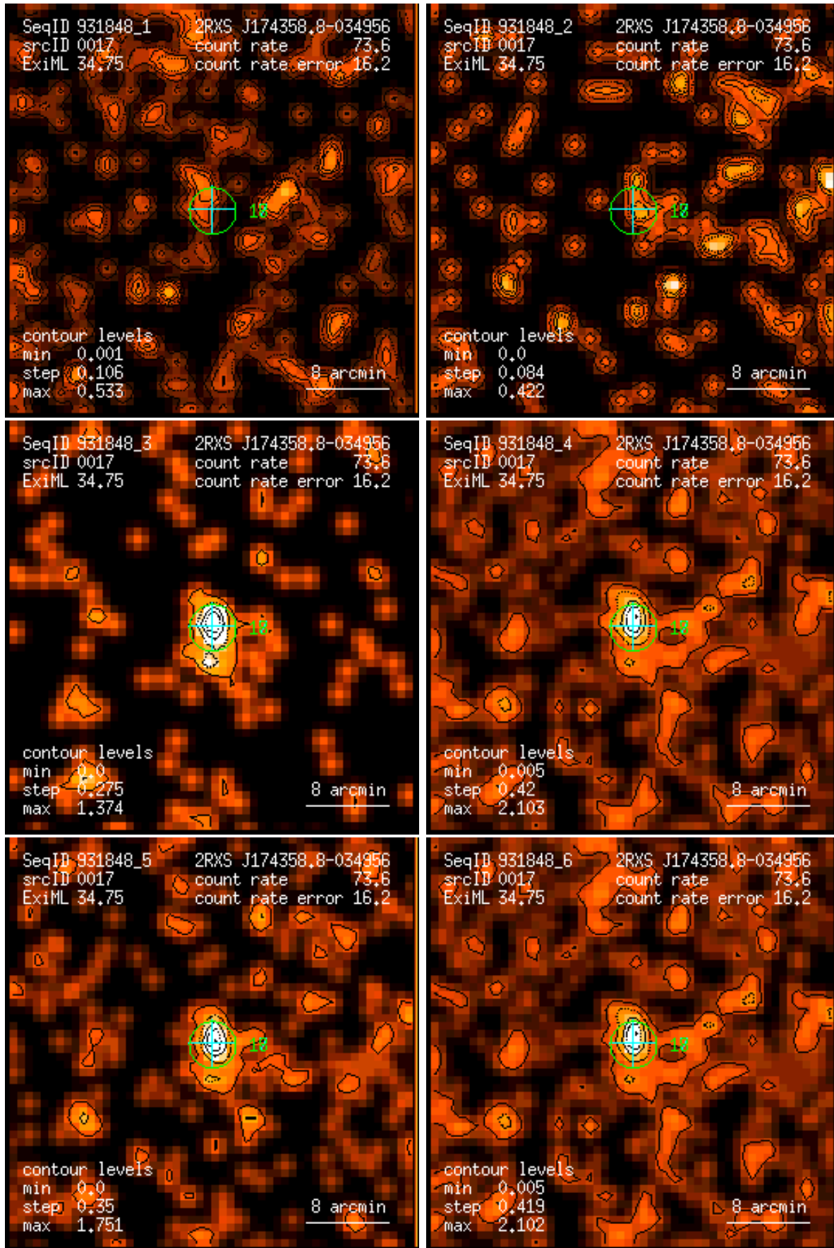
Figure 17: RASS 931848: detection 0017: band rate images, Gaussian filter: (1) PSPC channels 11 – 41, (2) 52 – 90, (3) 91 – 201, (4) 11 – 235, (5) 52 – 201, (6) 11 – 201. Broad band rates in counts/ks. Band rate contour levels in counts/ks/arcmin 2 .
