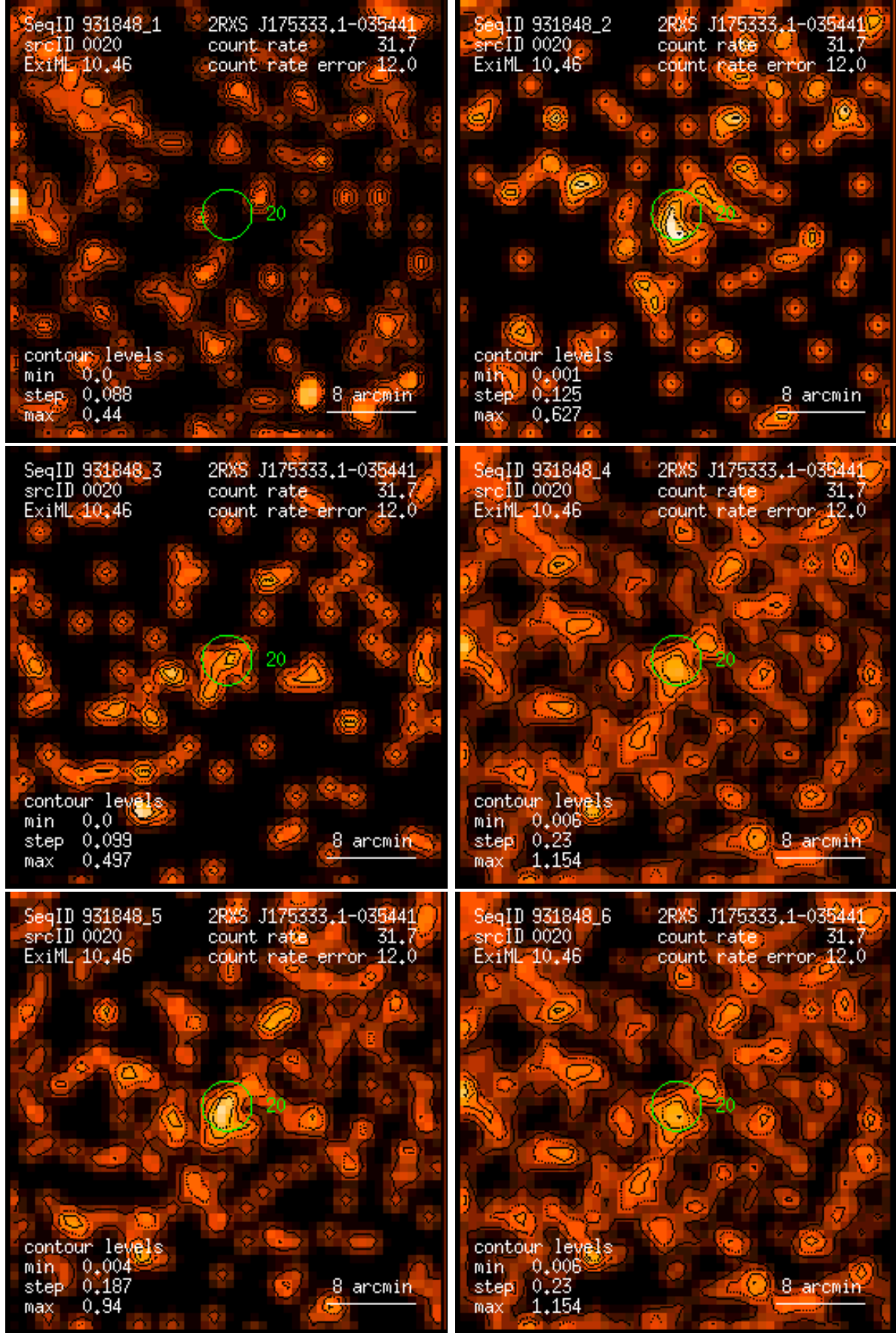
Figure 20: RASS 931848: detection 0020: band rate images, Gaussian filter: (1) PSPC channels 11 – 41, (2) 52 – 90, (3) 91 – 201, (4) 11 – 235, (5) 52 – 201, (6) 11 – 201. Broad band rates in counts/ks. Band rate contour levels in counts/ks/arcmin 2 .
