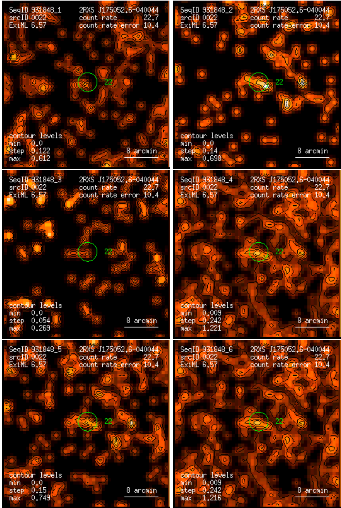
Figure 22: RASS 931848: detection 0022: band rate images, Gaussian filter: (1) PSPC channels 11 – 41, (2) 52 – 90, (3) 91 – 201, (4) 11 – 235, (5) 52 – 201, (6) 11 – 201. Broad band rates in counts/ks. Band rate contour levels in counts/ks/arcmin 2 .
