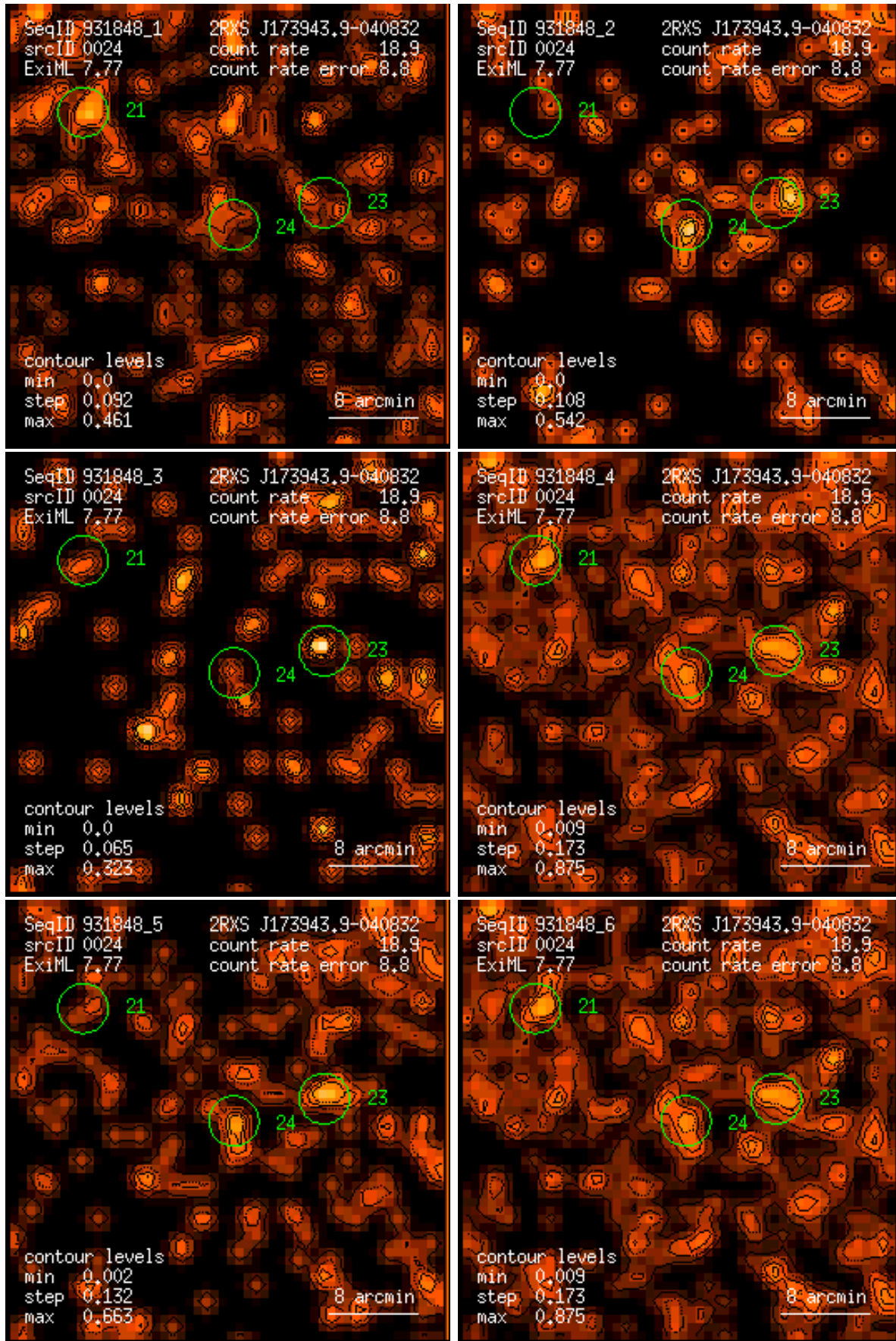
Figure 24: RASS 931848: detection 0024: band rate images, Gaussian filter: (1) PSPC channels 11 – 41, (2) 52 – 90, (3) 91 – 201, (4) 11 – 235, (5) 52 – 201, (6) 11 – 201. Broad band rates in counts/ks. Band rate contour levels in counts/ks/arcmin 2 .
