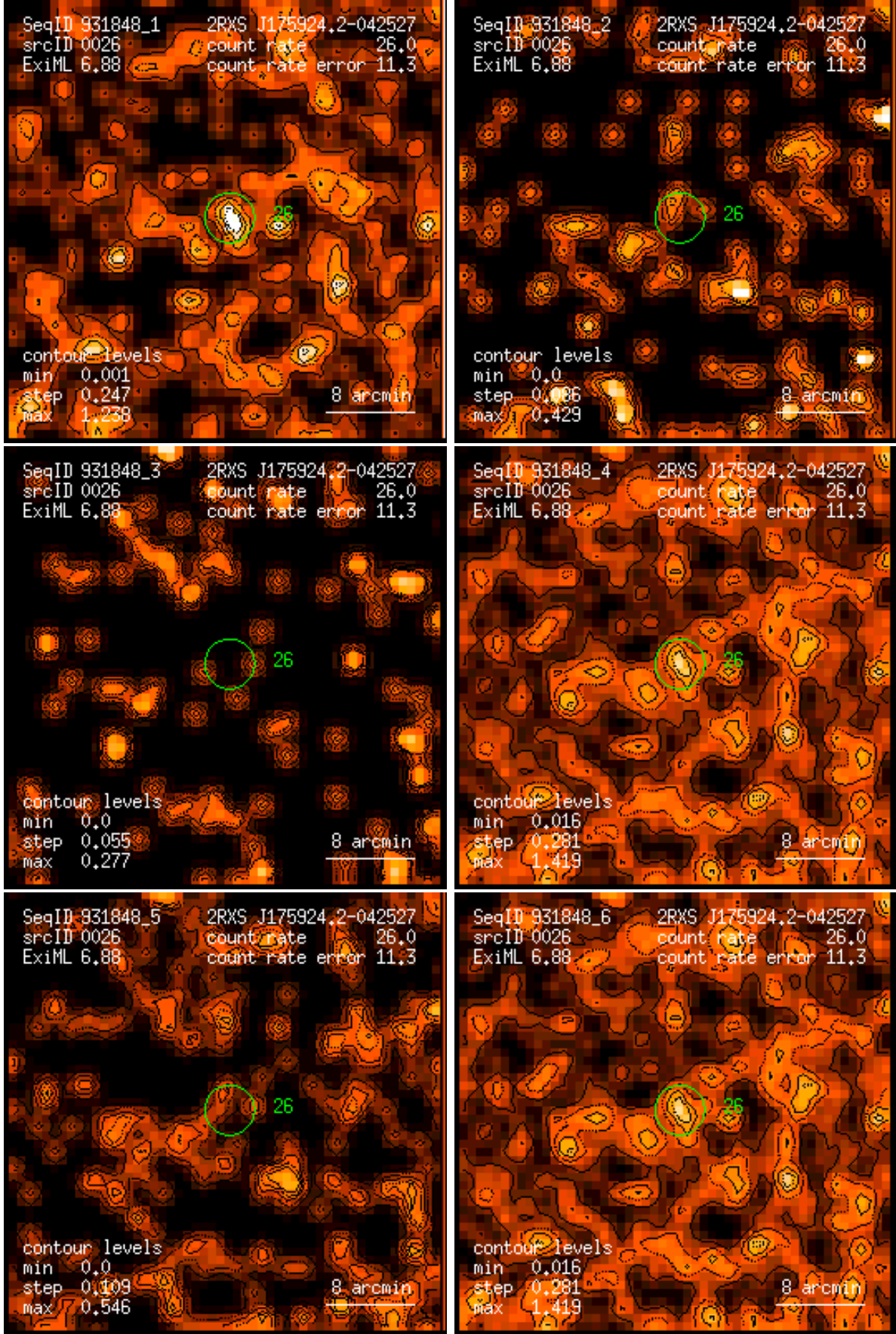
Figure 26: RASS 931848: detection 0026: band rate images, Gaussian filter: (1) PSPC channels 11 – 41, (2) 52 – 90, (3) 91 – 201, (4) 11 – 235, (5) 52 – 201, (6) 11 – 201. Broad band rates in counts/ks. Band rate contour levels in counts/ks/arcmin 2 .
