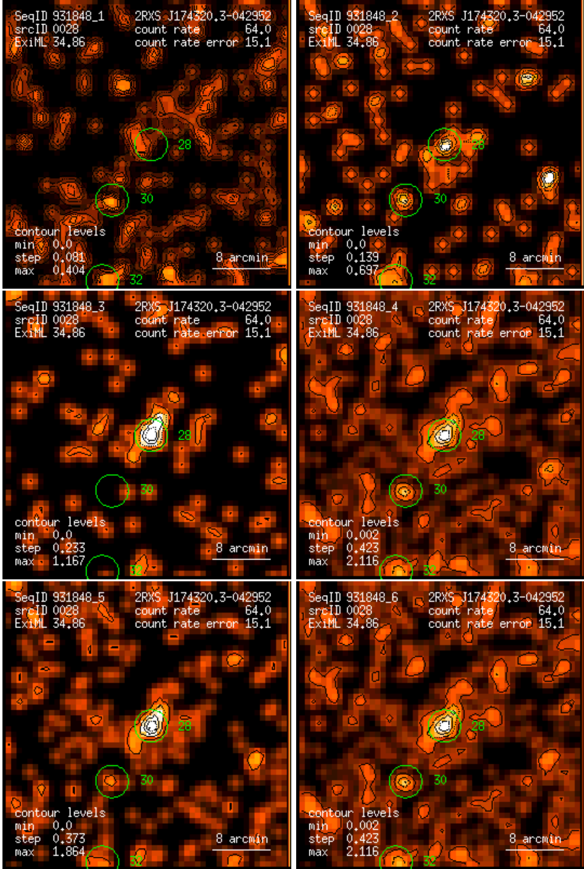
Figure 28: RASS 931848: detection 0028: band rate images, Gaussian filter: (1) PSPC channels 11 – 41, (2) 52 – 90, (3) 91 – 201, (4) 11 – 235, (5) 52 – 201, (6) 11 – 201. Broad band rates in counts/ks. Band rate contour levels in counts/ks/arcmin 2 .
