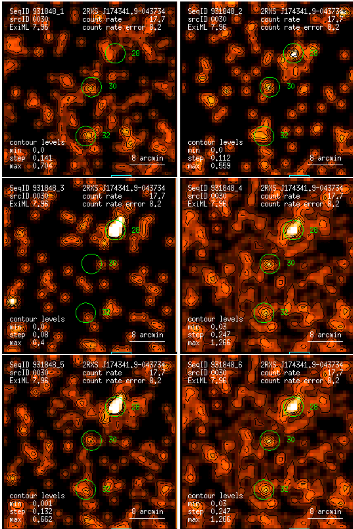
Figure 30: RASS 931848: detection 0030: band rate images, Gaussian filter: (1) PSPC channels 11 – 41, (2) 52 – 90, (3) 91 – 201, (4) 11 – 235, (5) 52 – 201, (6) 11 – 201. Broad band rates in counts/ks. Band rate contour levels in counts/ks/arcmin 2 .
