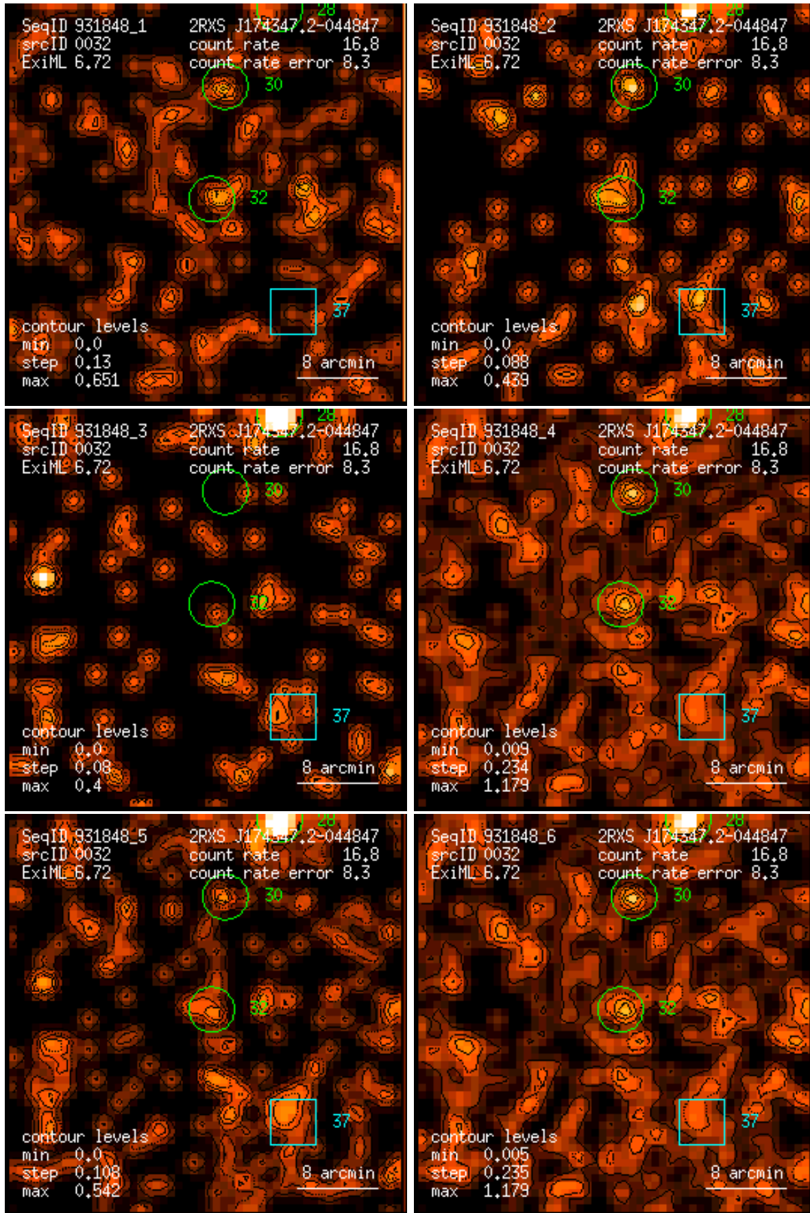
Figure 32: RASS 931848: detection 0032: band rate images, Gaussian filter: (1) PSPC channels 11 – 41, (2) 52 – 90, (3) 91 – 201, (4) 11 – 235, (5) 52 – 201, (6) 11 – 201. Broad band rates in counts/ks. Band rate contour levels in counts/ks/arcmin 2 .
