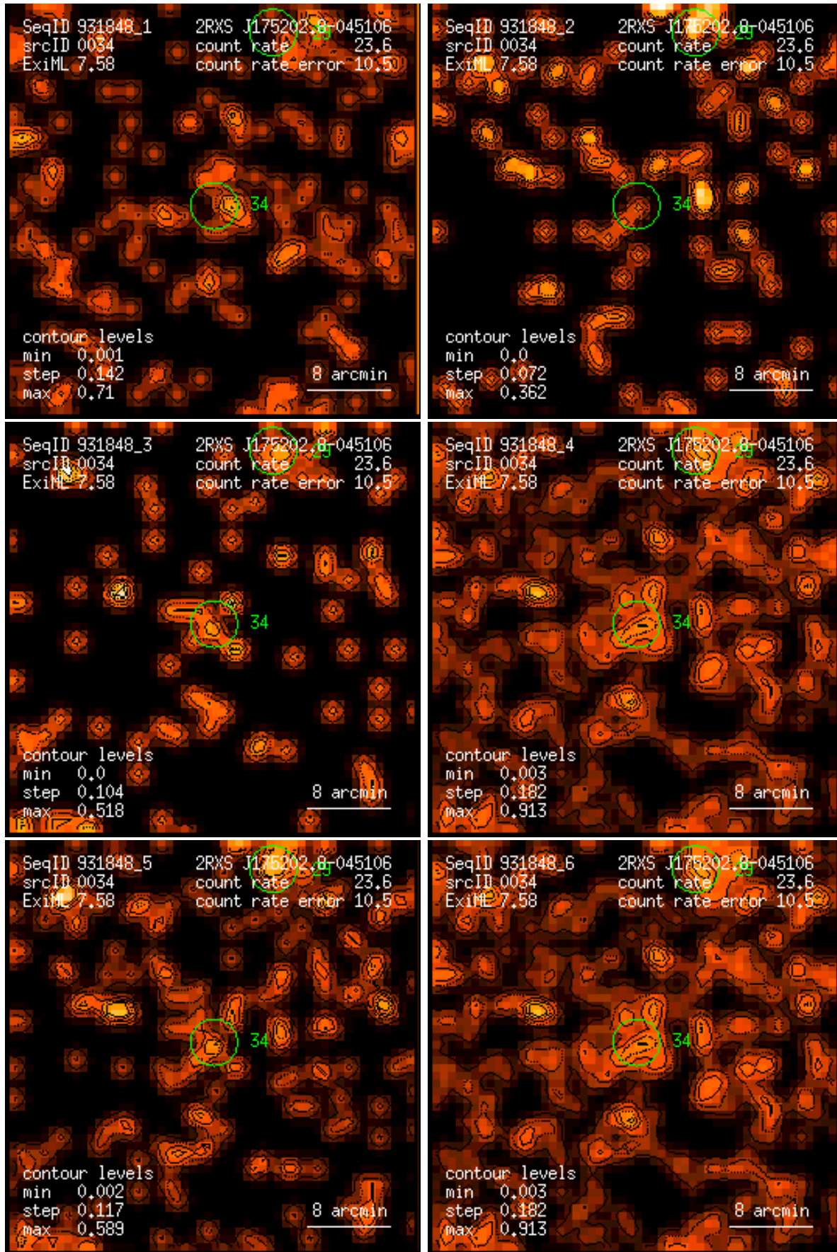
Figure 34: RASS 931848: detection 0034: band rate images, Gaussian filter: (1) PSPC channels 11 – 41, (2) 52 – 90, (3) 91 – 201, (4) 11 – 235, (5) 52 – 201, (6) 11 – 201. Broad band rates in counts/ks. Band rate contour levels in counts/ks/arcmin 2 .
