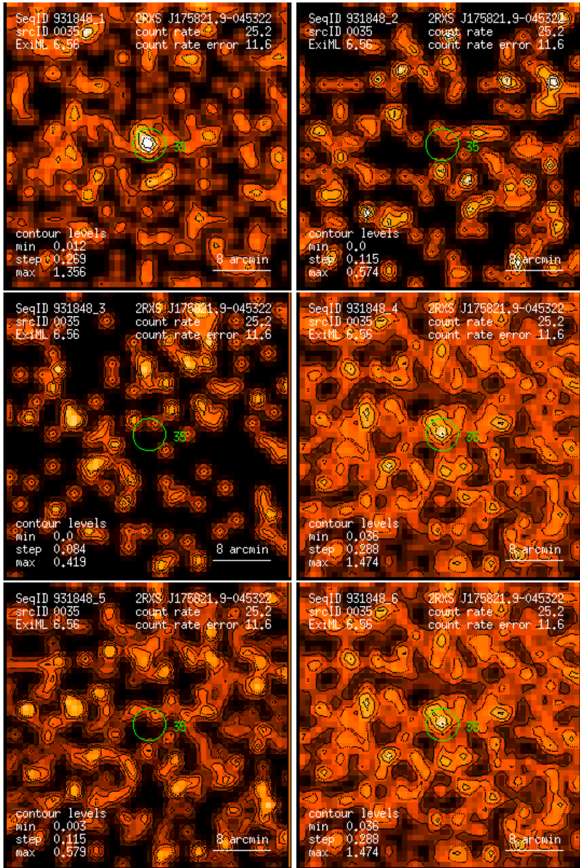
Figure 35: RASS 931848: detection 0035: band rate images, Gaussian filter: (1) PSPC channels 11 – 41, (2) 52 – 90, (3) 91 – 201, (4) 11 – 235, (5) 52 – 201, (6) 11 – 201. Broad band rates in counts/ks. Band rate contour levels in counts/ks/arcmin 2 .
