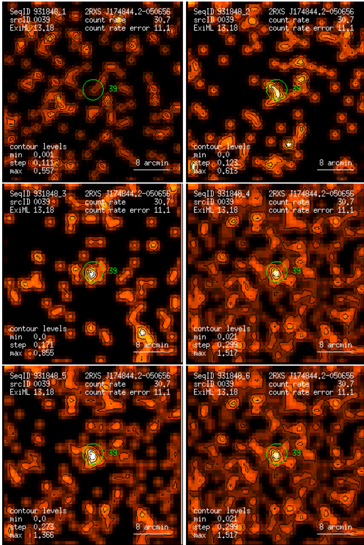
Figure 39: RASS 931848: detection 0039: band rate images, Gaussian filter: (1) PSPC channels 11 – 41, (2) 52 – 90, (3) 91 – 201, (4) 11 – 235, (5) 52 – 201, (6) 11 – 201. Broad band rates in counts/ks. Band rate contour levels in counts/ks/arcmin 2 .
