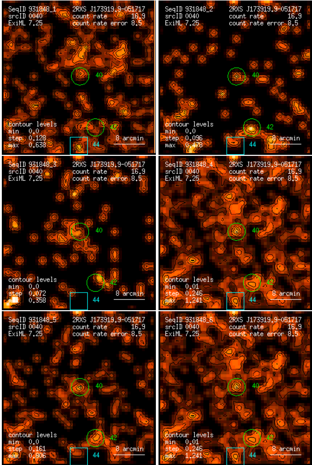
Figure 40: RASS 931848: detection 0040: band rate images, Gaussian filter: (1) PSPC channels 11 – 41, (2) 52 – 90, (3) 91 – 201, (4) 11 – 235, (5) 52 – 201, (6) 11 – 201. Broad band rates in counts/ks. Band rate contour levels in counts/ks/arcmin 2 .
