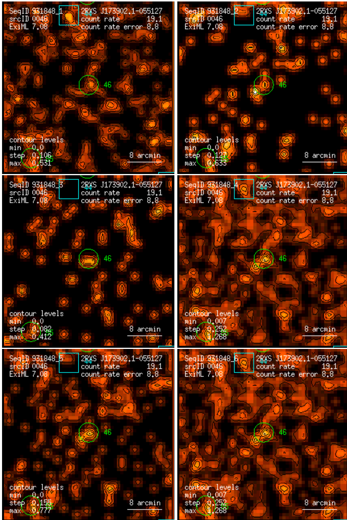
Figure 46: RASS 931848: detection 0046: band rate images, Gaussian filter: (1) PSPC channels 11 – 41, (2) 52 – 90, (3) 91 – 201, (4) 11 – 235, (5) 52 – 201, (6) 11 – 201. Broad band rates in counts/ks. Band rate contour levels in counts/ks/arcmin 2 .
