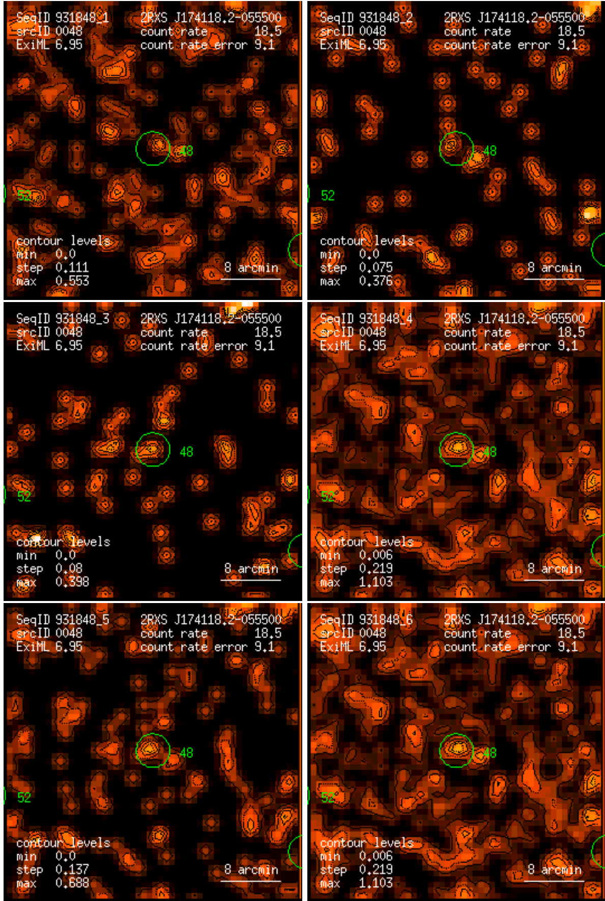
Figure 48: RASS 931848: detection 0048: band rate images, Gaussian filter: (1) PSPC channels 11 – 41, (2) 52 – 90, (3) 91 – 201, (4) 11 – 235, (5) 52 – 201, (6) 11 – 201. Broad band rates in counts/ks. Band rate contour levels in counts/ks/arcmin 2 .
