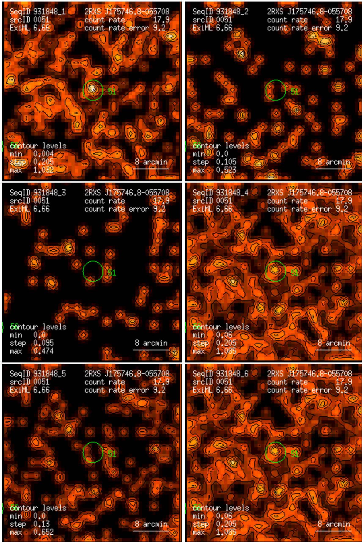
Figure 51: RASS 931848: detection 0051: band rate images, Gaussian filter: (1) PSPC channels 11 – 41, (2) 52 – 90, (3) 91 – 201, (4) 11 – 235, (5) 52 – 201, (6) 11 – 201. Broad band rates in counts/ks. Band rate contour levels in counts/ks/arcmin 2 .
