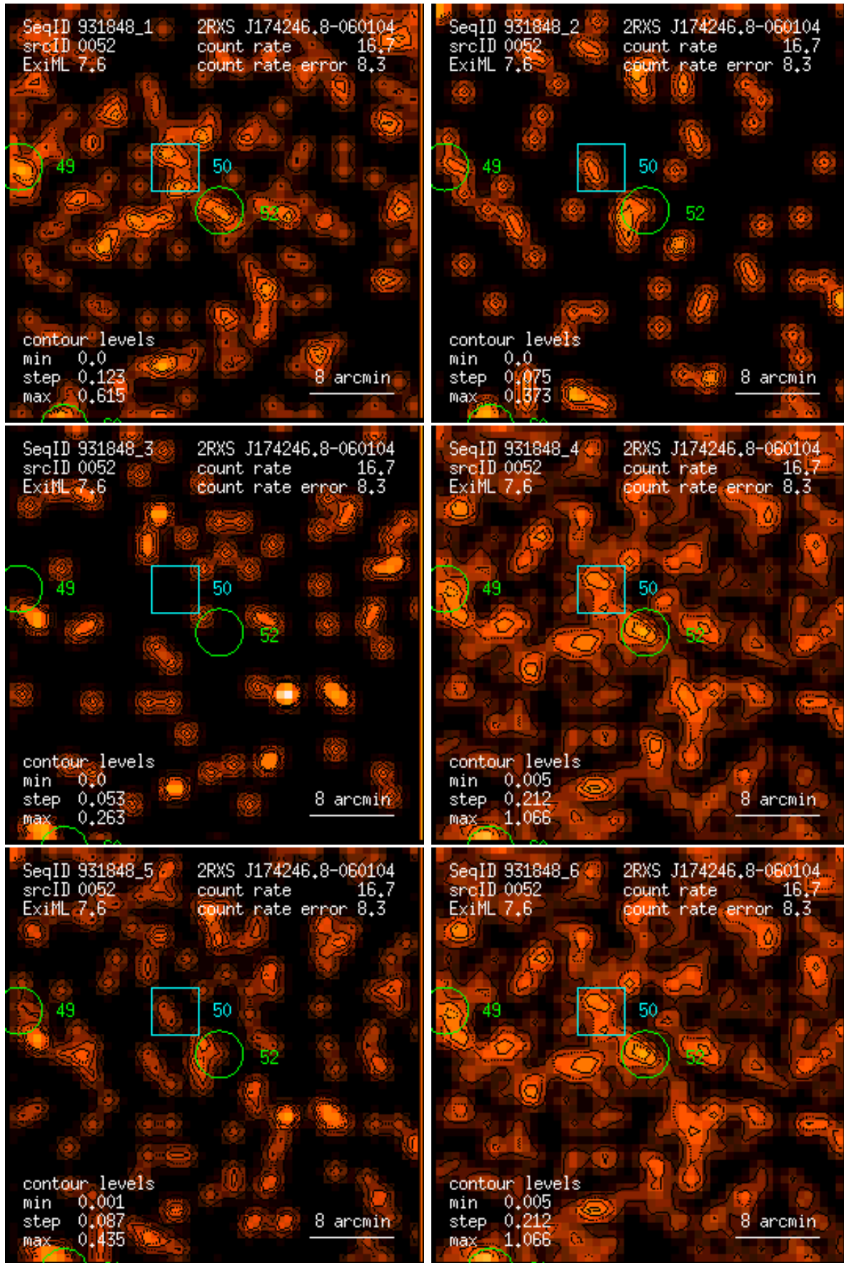
Figure 52: RASS 931848: detection 0052: band rate images, Gaussian filter: (1) PSPC channels 11 – 41, (2) 52 – 90, (3) 91 – 201, (4) 11 – 235, (5) 52 – 201, (6) 11 – 201. Broad band rates in counts/ks. Band rate contour levels in counts/ks/arcmin 2 .
