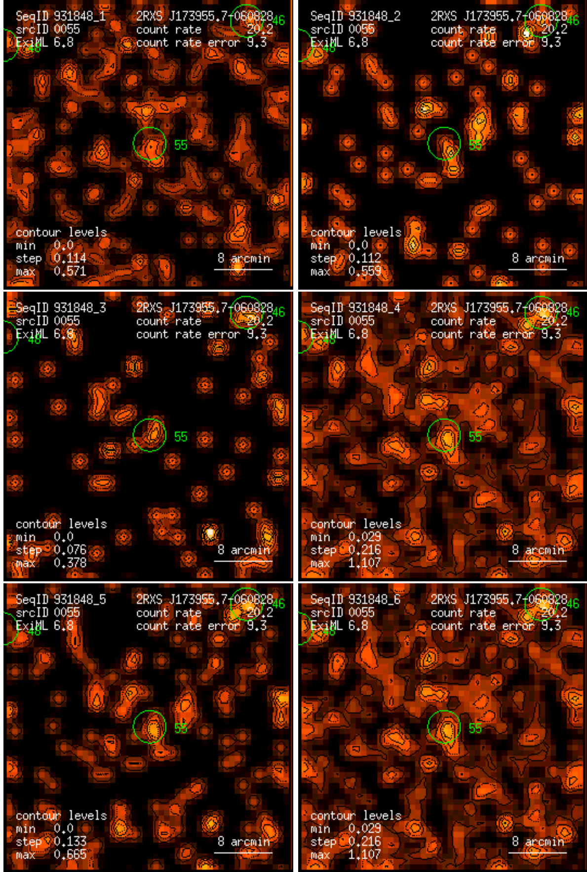
Figure 55: RASS 931848: detection 0055: band rate images, Gaussian filter: (1) PSPC channels 11 – 41, (2) 52 – 90, (3) 91 – 201, (4) 11 – 235, (5) 52 – 201, (6) 11 – 201. Broad band rates in counts/ks. Band rate contour levels in counts/ks/arcmin 2 .
