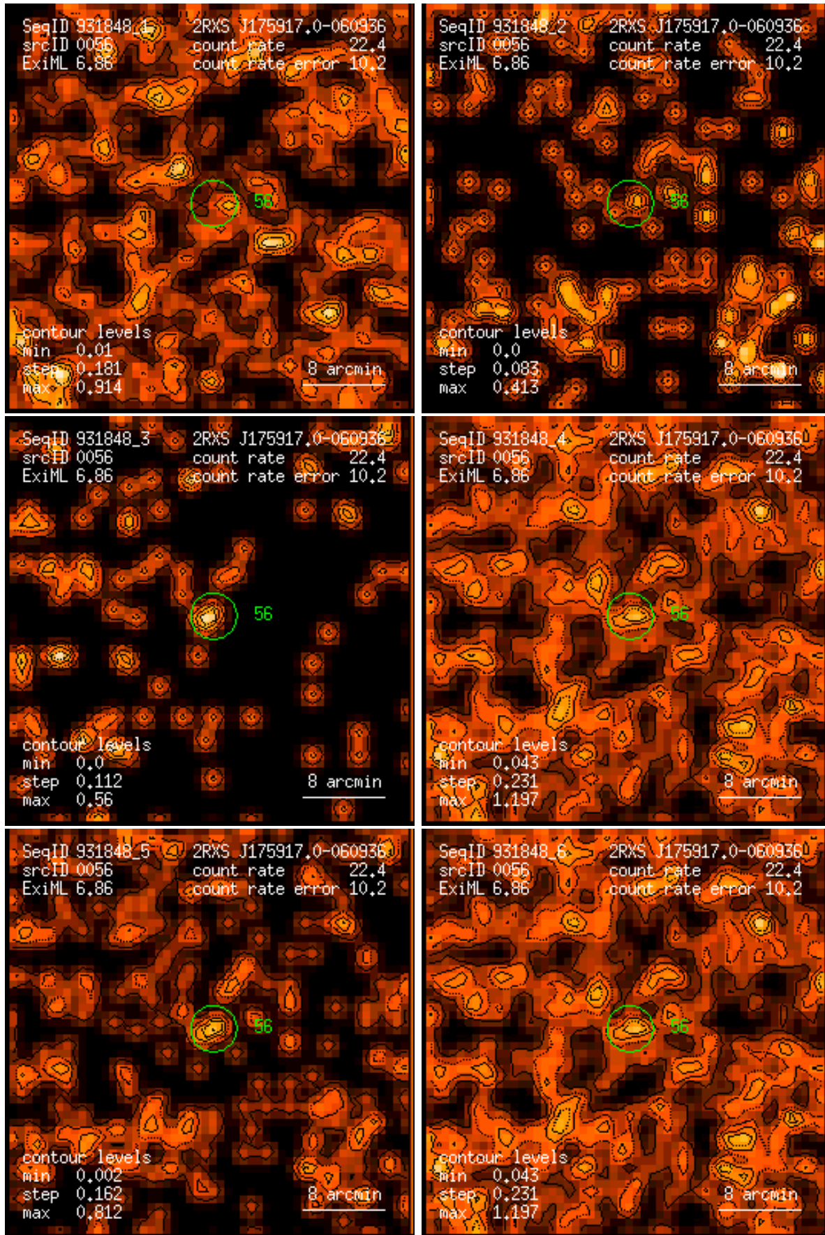
Figure 56: RASS 931848: detection 0056: band rate images, Gaussian filter: (1) PSPC channels 11 – 41, (2) 52 – 90, (3) 91 – 201, (4) 11 – 235, (5) 52 – 201, (6) 11 – 201. Broad band rates in counts/ks. Band rate contour levels in counts/ks/arcmin 2 .
