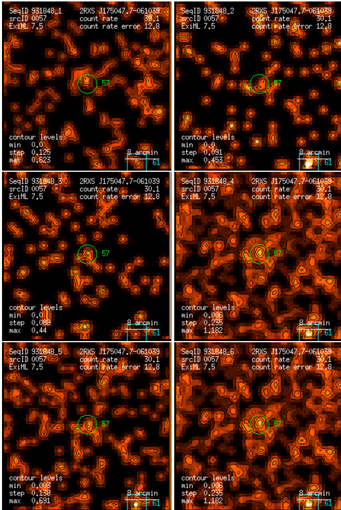
Figure 57: RASS 931848: detection 0057: band rate images, Gaussian filter: (1) PSPC channels 11 – 41, (2) 52 – 90, (3) 91 – 201, (4) 11 – 235, (5) 52 – 201, (6) 11 – 201. Broad band rates in counts/ks. Band rate contour levels in counts/ks/arcmin 2 .
