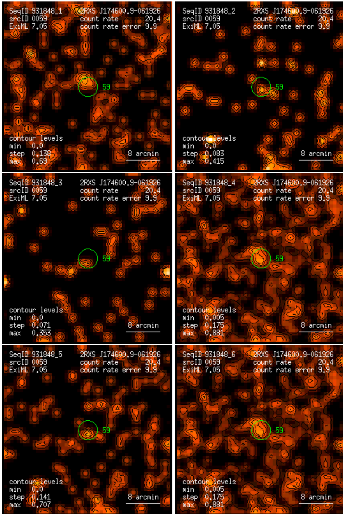
Figure 59: RASS 931848: detection 0059: band rate images, Gaussian filter: (1) PSPC channels 11 – 41, (2) 52 – 90, (3) 91 – 201, (4) 11 – 235, (5) 52 – 201, (6) 11 – 201. Broad band rates in counts/ks. Band rate contour levels in counts/ks/arcmin 2 .
