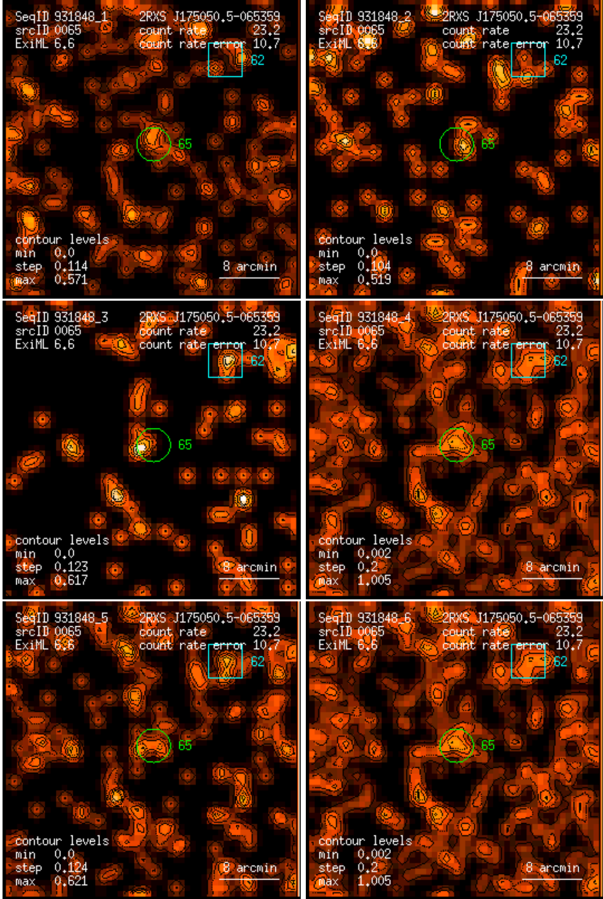
Figure 65: RASS 931848: detection 0065: band rate images, Gaussian filter: (1) PSPC channels 11 – 41, (2) 52 – 90, (3) 91 – 201, (4) 11 – 235, (5) 52 – 201, (6) 11 – 201. Broad band rates in counts/ks. Band rate contour levels in counts/ks/arcmin 2 .
