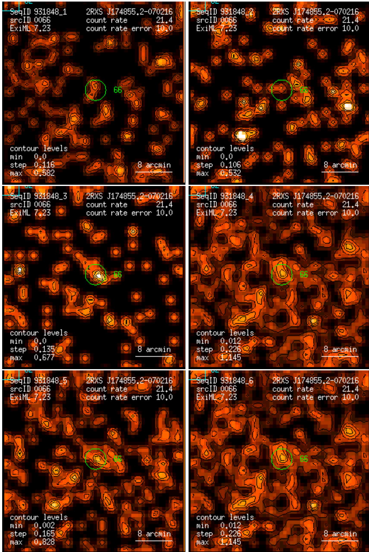
Figure 66: RASS 931848: detection 0066: band rate images, Gaussian filter: (1) PSPC channels 11 – 41, (2) 52 – 90, (3) 91 – 201, (4) 11 – 235, (5) 52 – 201, (6) 11 – 201. Broad band rates in counts/ks. Band rate contour levels in counts/ks/arcmin 2 .
