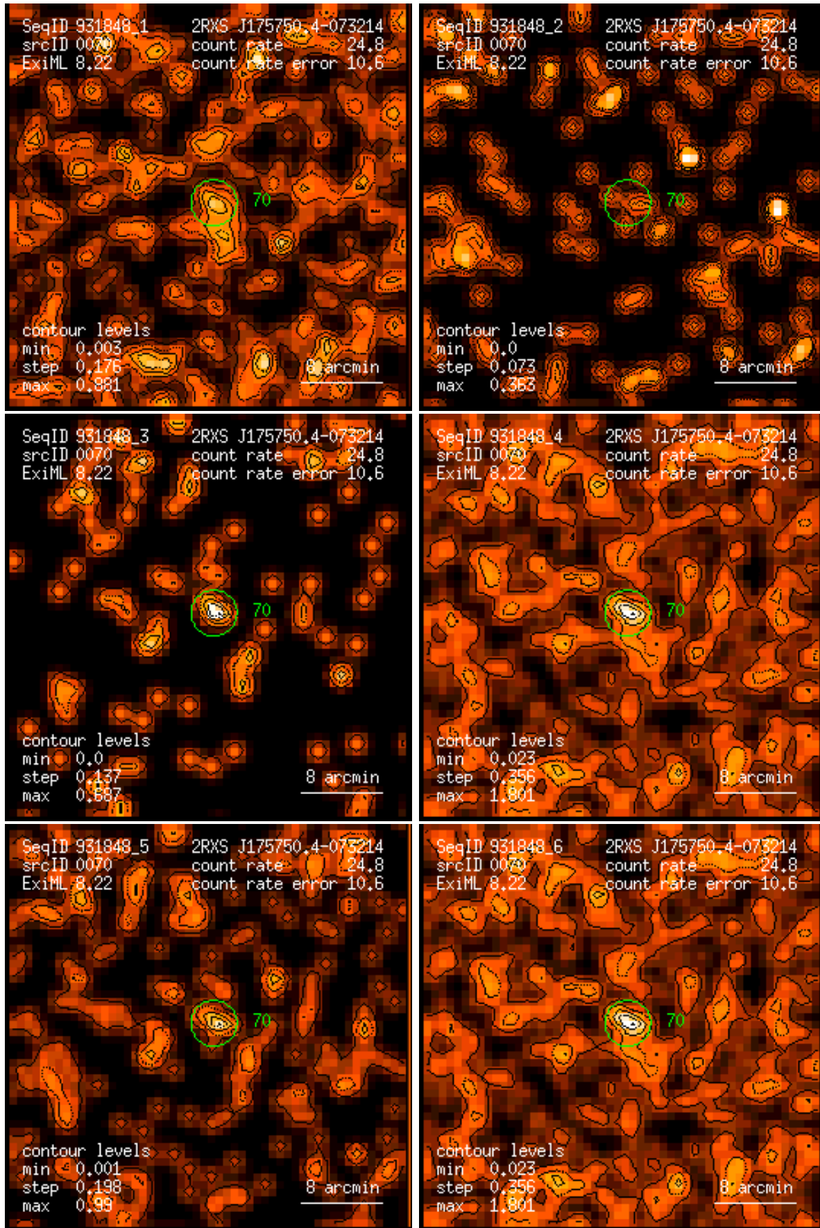
Figure 70: RASS 931848: detection 0070: band rate images, Gaussian filter: (1) PSPC channels 11 – 41, (2) 52 – 90, (3) 91 – 201, (4) 11 – 235, (5) 52 – 201, (6) 11 – 201. Broad band rates in counts/ks. Band rate contour levels in counts/ks/arcmin 2 .
