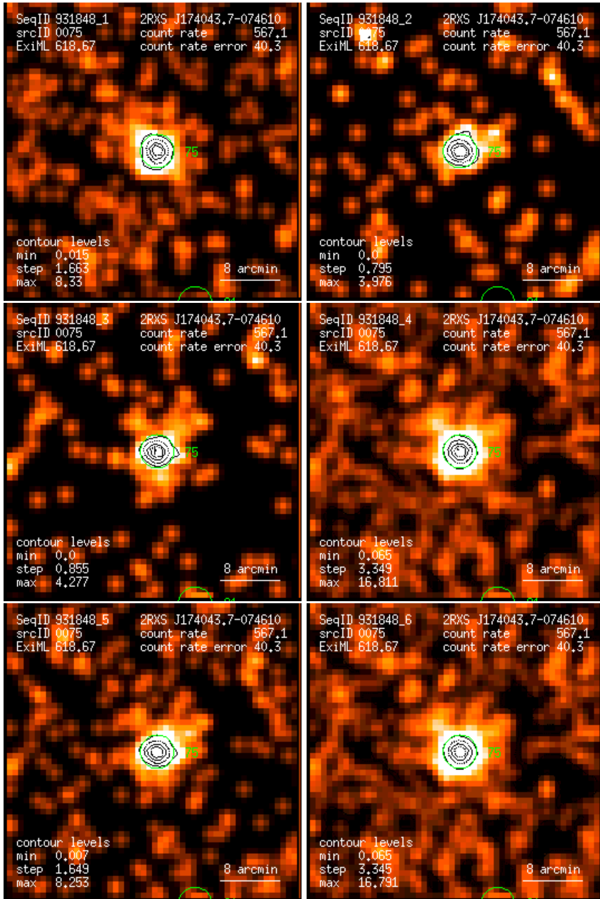
Figure 75: RASS 931848: detection 0075: band rate images, Gaussian filter: (1) PSPC channels 11 – 41, (2) 52 – 90, (3) 91 – 201, (4) 11 – 235, (5) 52 – 201, (6) 11 – 201. Broad band rates in counts/ks. Band rate contour levels in counts/ks/arcmin 2 .
