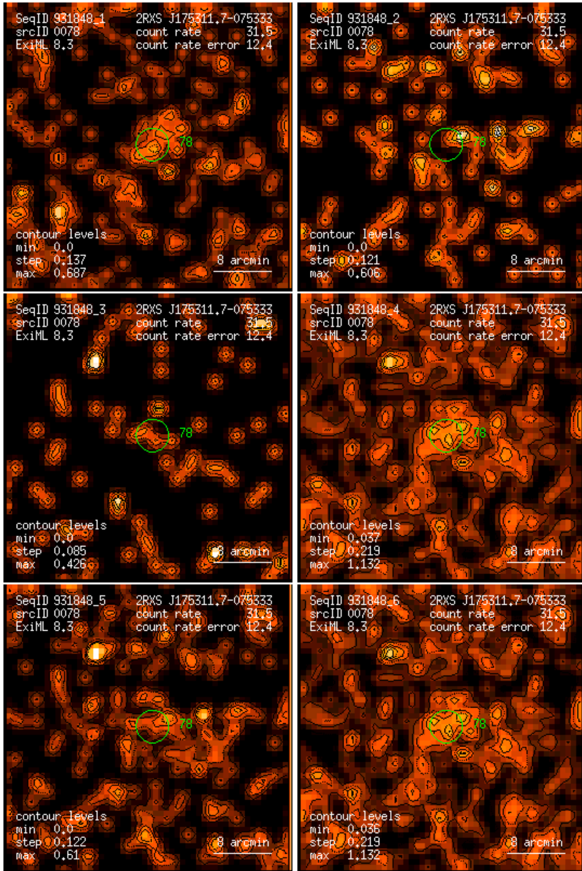
Figure 78: RASS 931848: detection 0078: band rate images, Gaussian filter: (1) PSPC channels 11 – 41, (2) 52 – 90, (3) 91 – 201, (4) 11 – 235, (5) 52 – 201, (6) 11 – 201. Broad band rates in counts/ks. Band rate contour levels in counts/ks/arcmin 2 .
